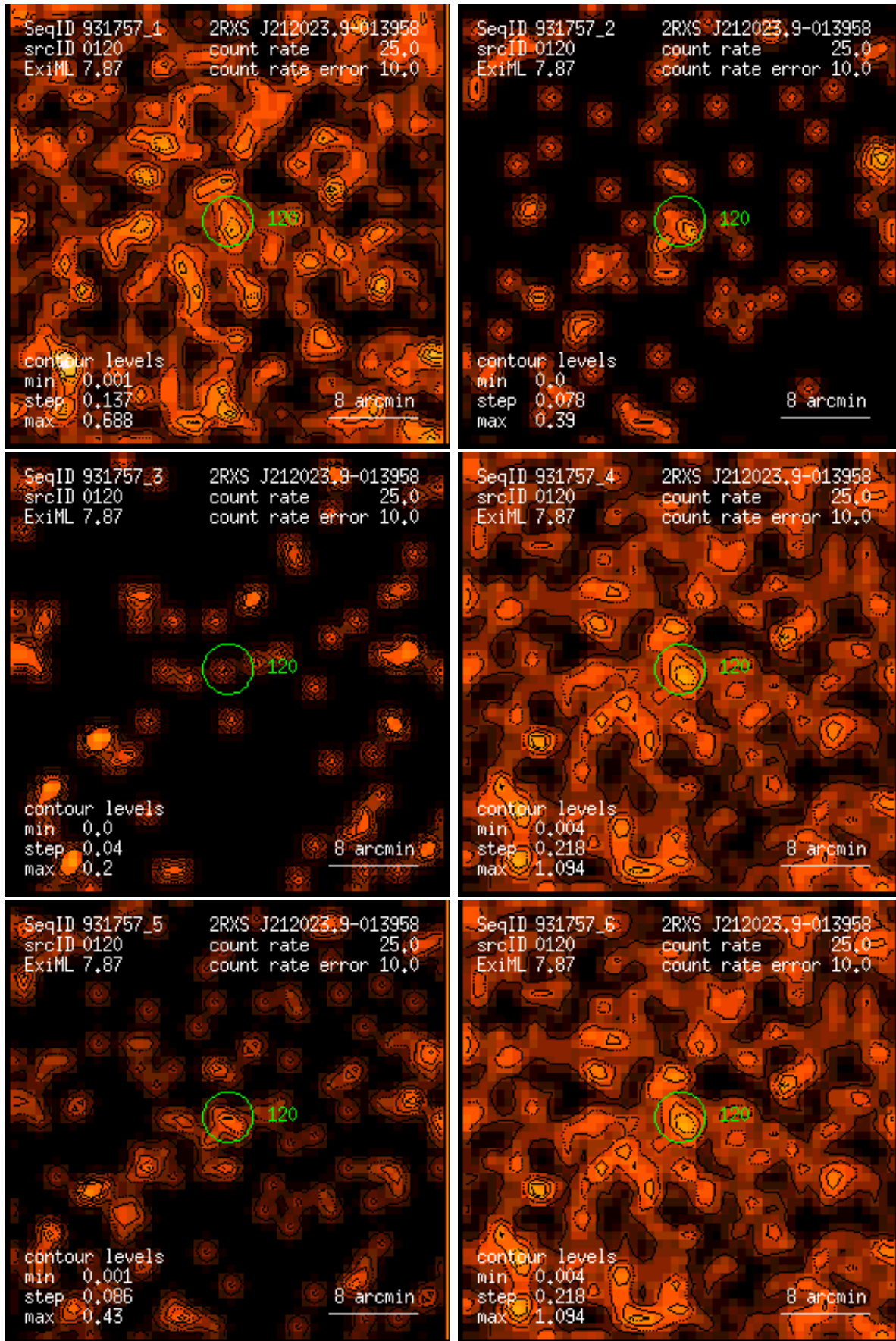
Figure 120: RASS 931757: detection 0120: band rate images, Gaussian filter: (1) PSPC channels 11 – 41, (2) 52 – 90, (3) 91 – 201, (4) 11 – 235, (5) 52 – 201, (6) 11 – 201. Broad band rates in counts/ks. Band rate contour levels in counts/ks/arcmin 2 .
