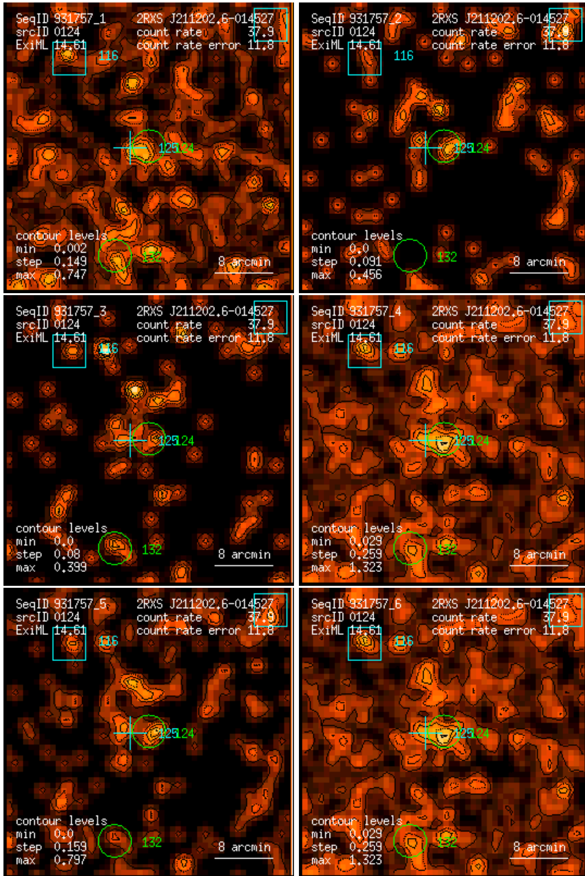
Figure 124: RASS 931757: detection 0124: band rate images, Gaussian filter: (1) PSPC channels 11 – 41, (2) 52 – 90, (3) 91 – 201, (4) 11 – 235, (5) 52 – 201, (6) 11 – 201. Broad band rates in counts/ks. Band rate contour levels in counts/ks/arcmin 2 .
