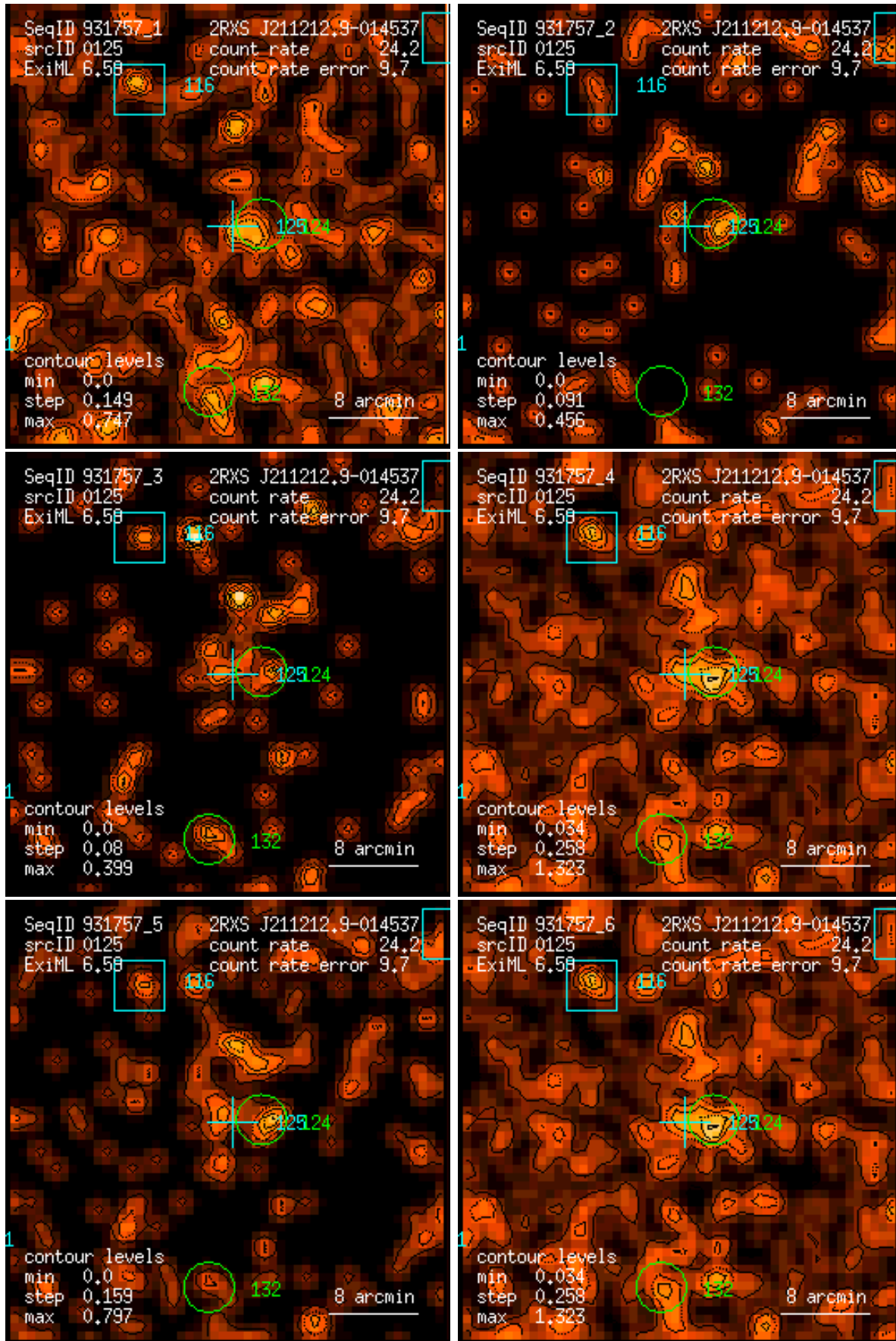
Figure 125: RASS 931757: detection 0125: band rate images, Gaussian filter: (1) PSPC channels 11 – 41, (2) 52 – 90, (3) 91 – 201, (4) 11 – 235, (5) 52 – 201, (6) 11 – 201. Broad band rates in counts/ks. Band rate contour levels in counts/ks/arcmin 2 .
