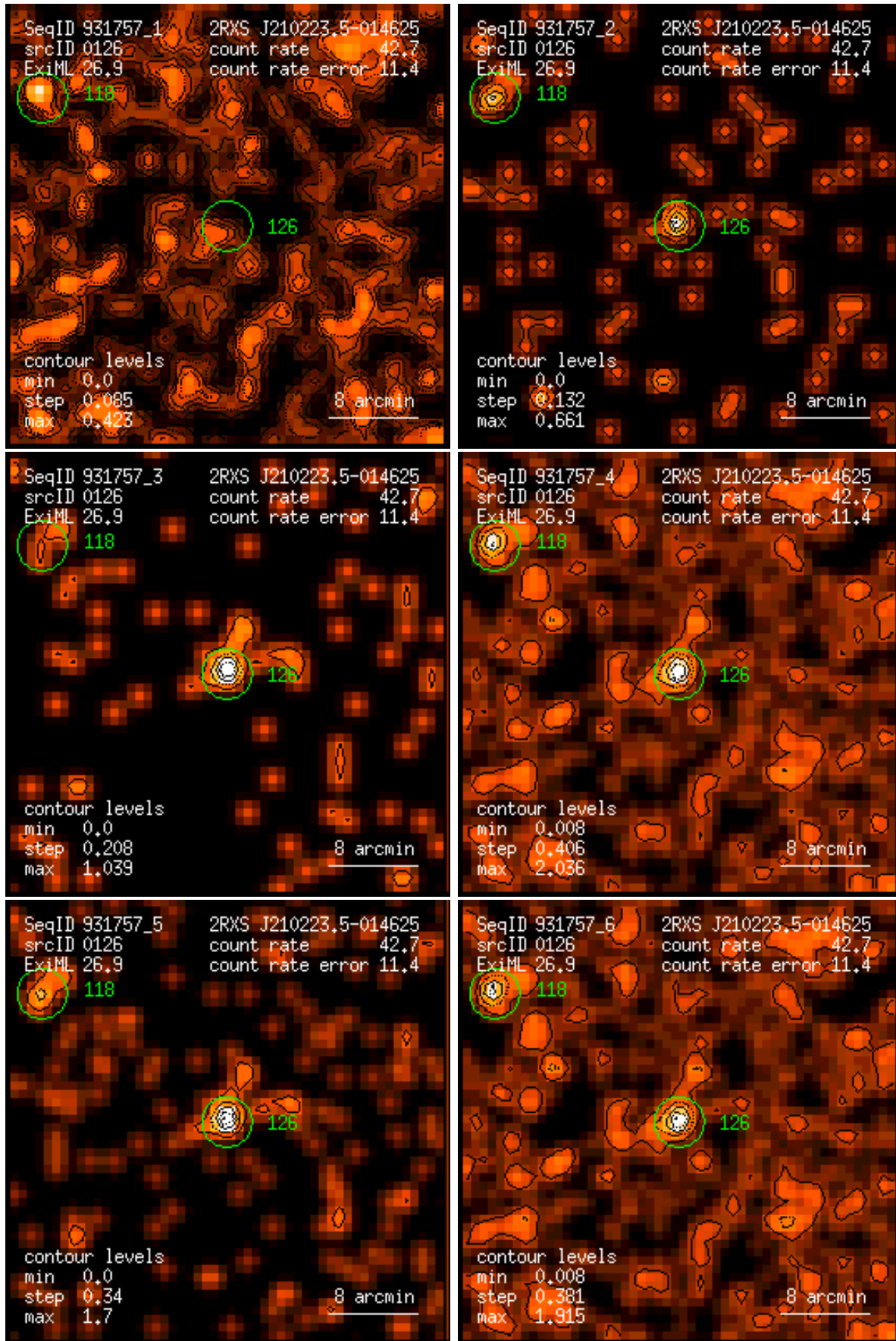
Figure 126: RASS 931757: detection 0126: band rate images, Gaussian filter: (1) PSPC channels 11 – 41, (2) 52 – 90, (3) 91 – 201, (4) 11 – 235, (5) 52 – 201, (6) 11 – 201. Broad band rates in counts/ks. Band rate contour levels in counts/ks/arcmin 2 .
