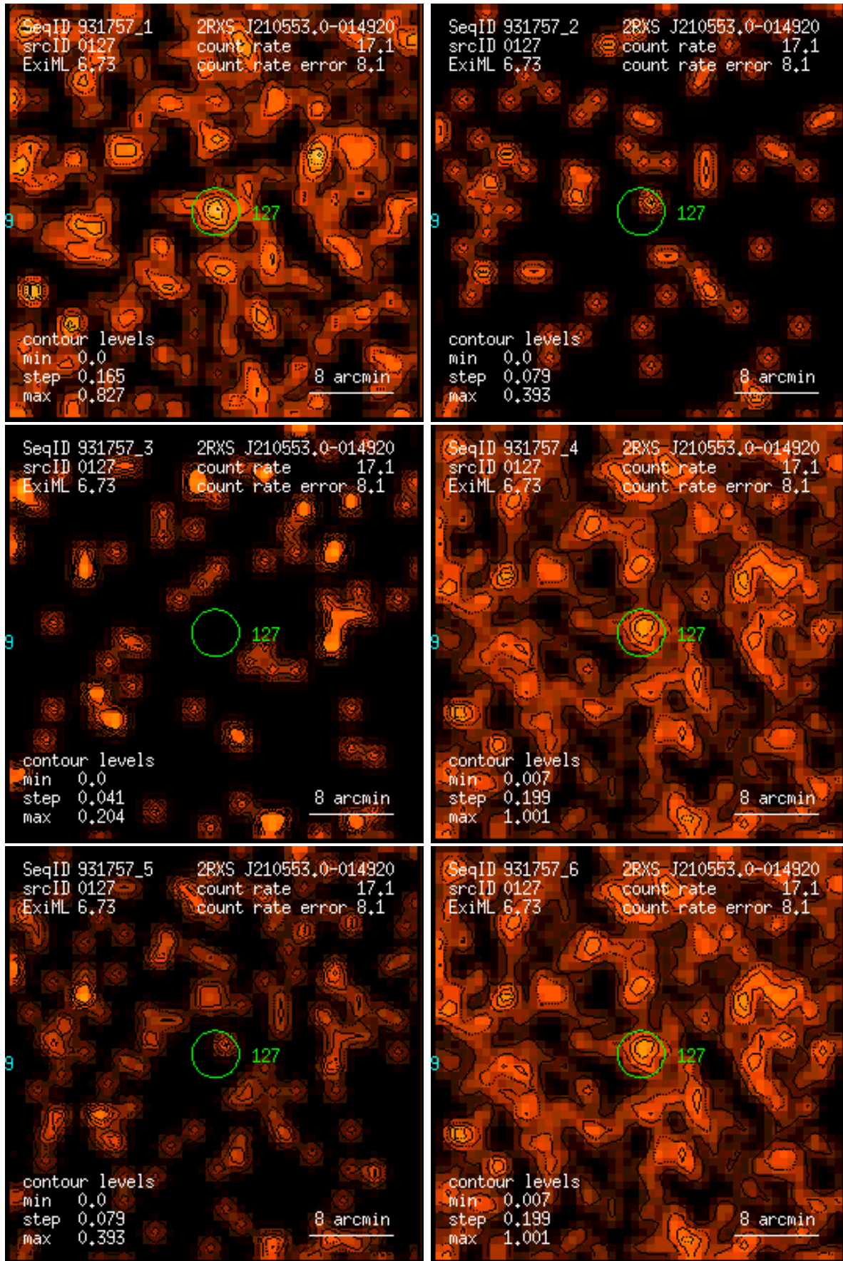
Figure 127: RASS 931757: detection 0127: band rate images, Gaussian filter: (1) PSPC channels 11 – 41, (2) 52 – 90, (3) 91 – 201, (4) 11 – 235, (5) 52 – 201, (6) 11 – 201. Broad band rates in counts/ks. Band rate contour levels in counts/ks/arcmin 2 .
