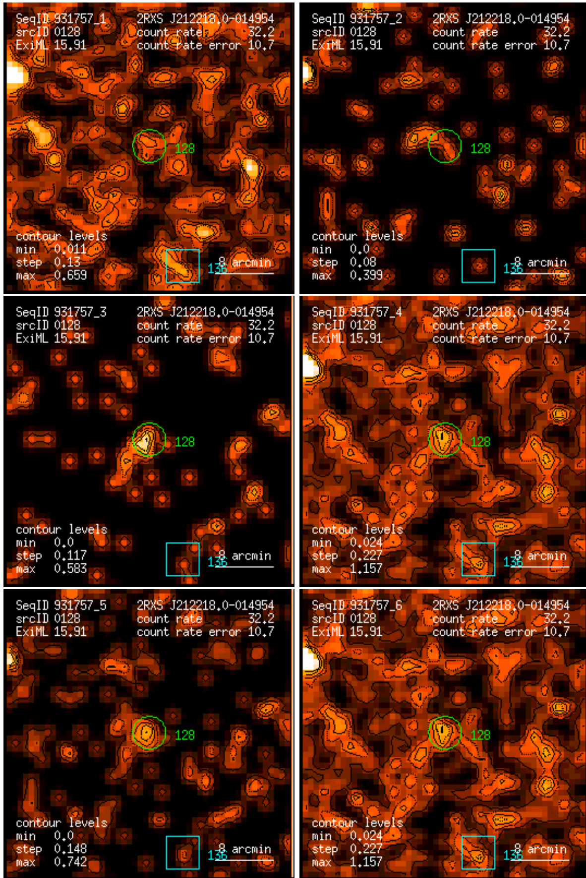
Figure 128: RASS 931757: detection 0128: band rate images, Gaussian filter: (1) PSPC channels 11 – 41, (2) 52 – 90, (3) 91 – 201, (4) 11 – 235, (5) 52 – 201, (6) 11 – 201. Broad band rates in counts/ks. Band rate contour levels in counts/ks/arcmin 2 .
