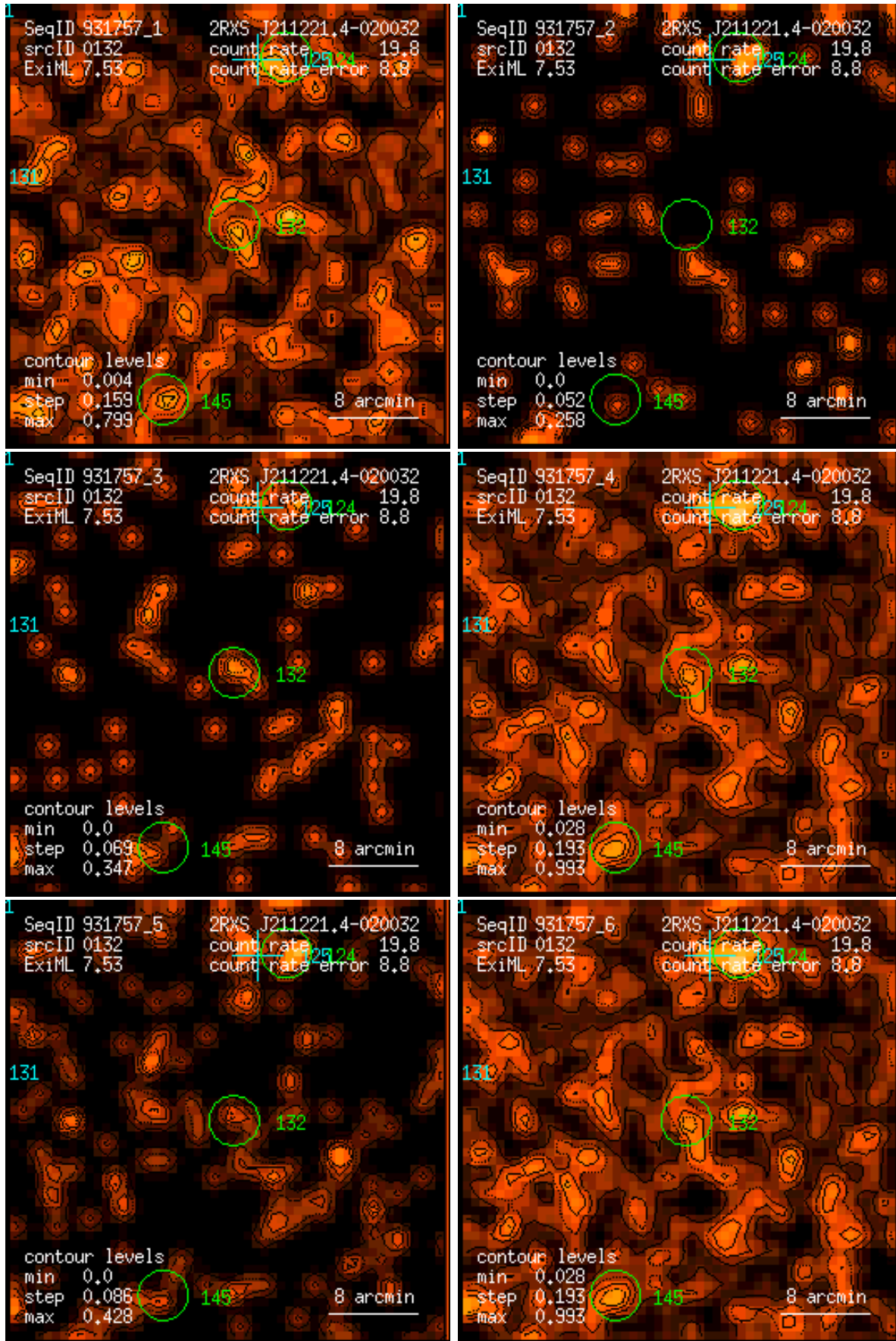
Figure 132: RASS 931757: detection 0132: band rate images, Gaussian filter: (1) PSPC channels 11 – 41, (2) 52 – 90, (3) 91 – 201, (4) 11 – 235, (5) 52 – 201, (6) 11 – 201. Broad band rates in counts/ks. Band rate contour levels in counts/ks/arcmin 2 .
