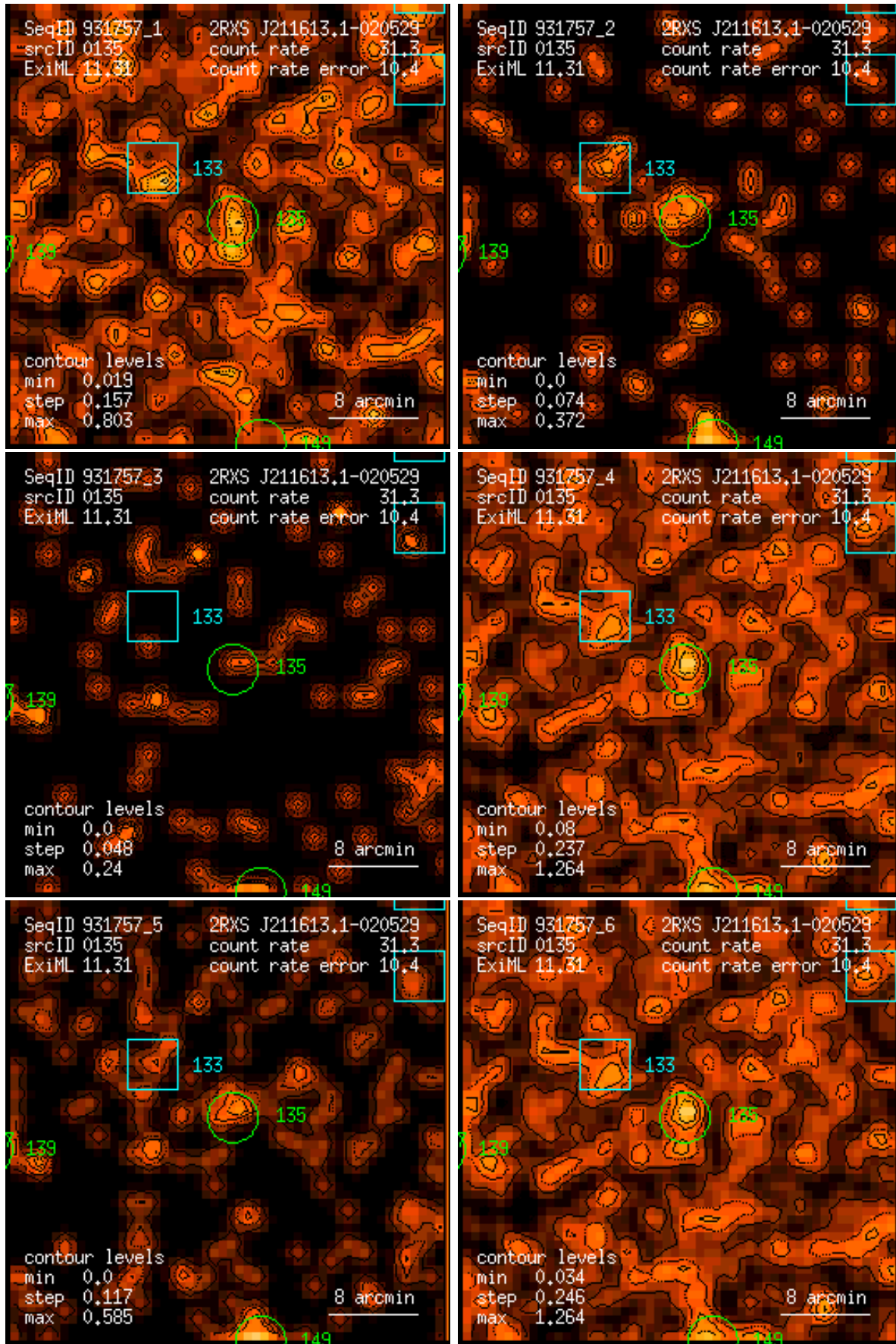
Figure 135: RASS 931757: detection 0135: band rate images, Gaussian filter: (1) PSPC channels 11 – 41, (2) 52 – 90, (3) 91 – 201, (4) 11 – 235, (5) 52 – 201, (6) 11 – 201. Broad band rates in counts/ks. Band rate contour levels in counts/ks/arcmin 2 .
