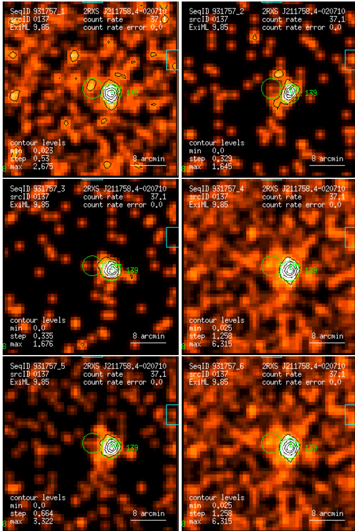
Figure 137: RASS 931757: detection 0137: band rate images, Gaussian filter: (1) PSPC channels 11 – 41, (2) 52 – 90, (3) 91 – 201, (4) 11 – 235, (5) 52 – 201, (6) 11 – 201. Broad band rates in counts/ks. Band rate contour levels in counts/ks/arcmin 2 .
