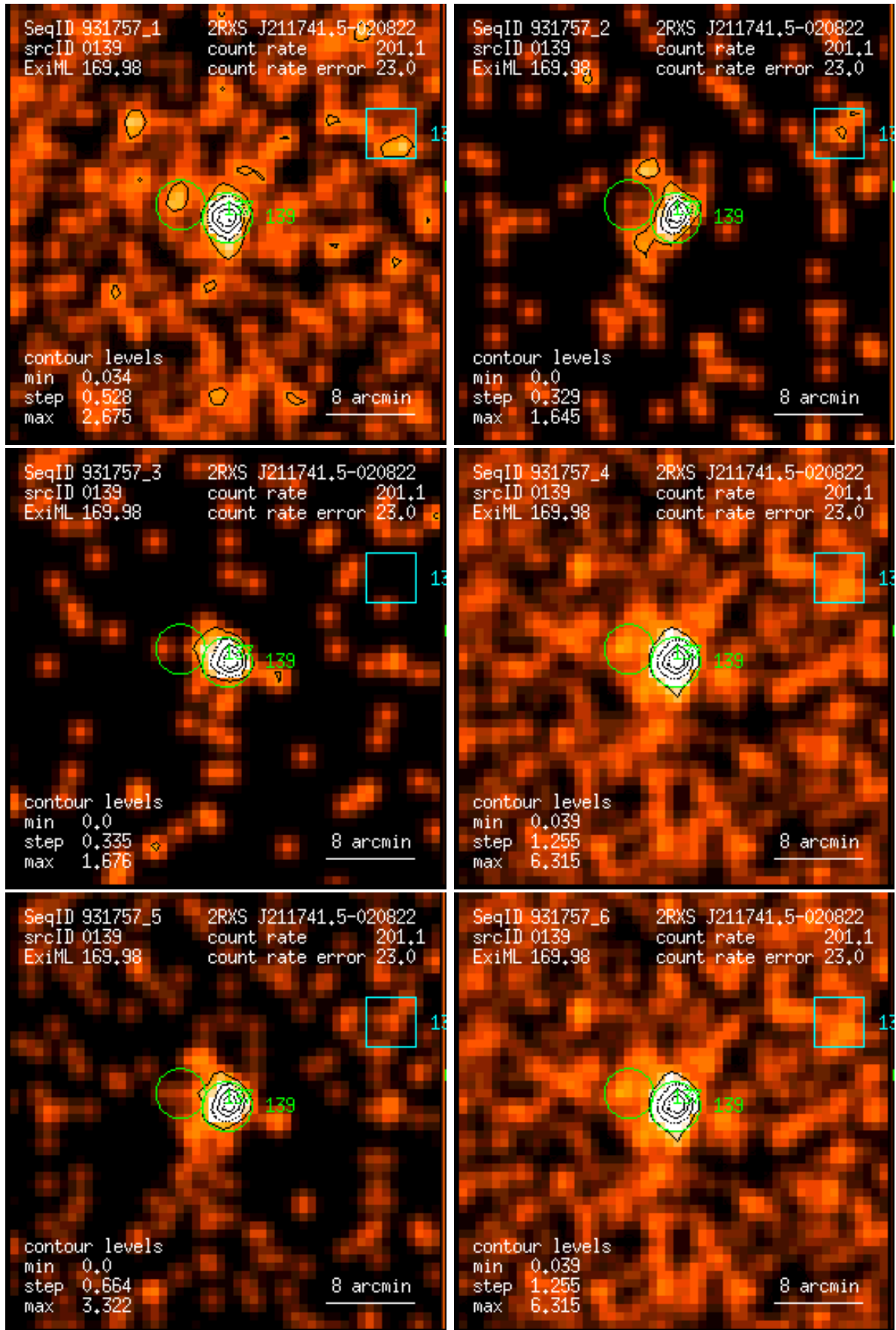
Figure 139: RASS 931757: detection 0139: band rate images, Gaussian filter: (1) PSPC channels 11 – 41, (2) 52 – 90, (3) 91 – 201, (4) 11 – 235, (5) 52 – 201, (6) 11 – 201. Broad band rates in counts/ks. Band rate contour levels in counts/ks/arcmin 2 .
