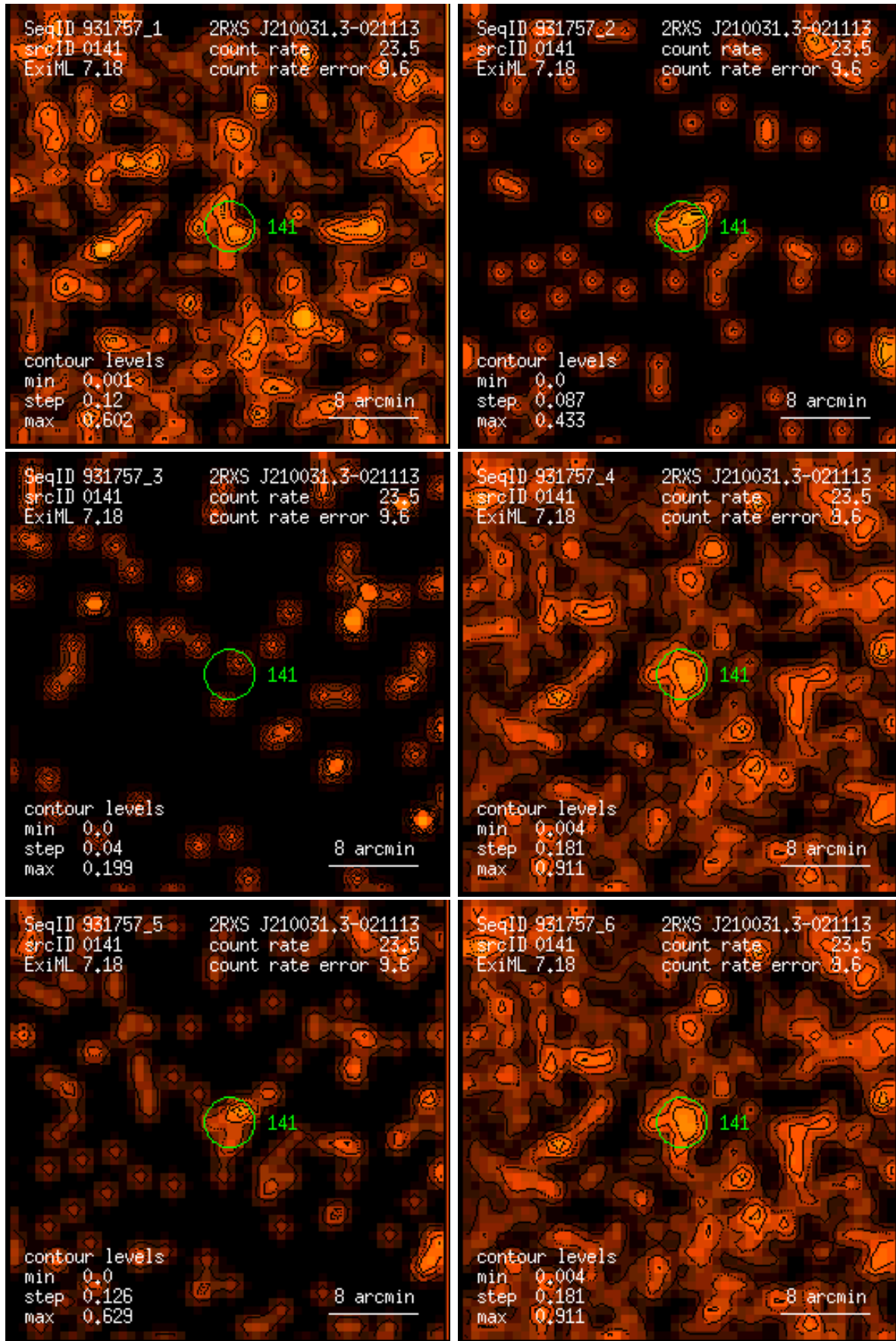
Figure 141: RASS 931757: detection 0141: band rate images, Gaussian filter: (1) PSPC channels 11 – 41, (2) 52 – 90, (3) 91 – 201, (4) 11 – 235, (5) 52 – 201, (6) 11 – 201. Broad band rates in counts/ks. Band rate contour levels in counts/ks/arcmin 2 .
