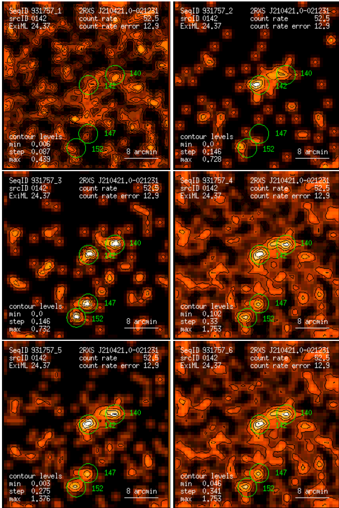
Figure 142: RASS 931757: detection 0142: band rate images, Gaussian filter: (1) PSPC channels 11 – 41, (2) 52 – 90, (3) 91 – 201, (4) 11 – 235, (5) 52 – 201, (6) 11 – 201. Broad band rates in counts/ks. Band rate contour levels in counts/ks/arcmin 2 .
