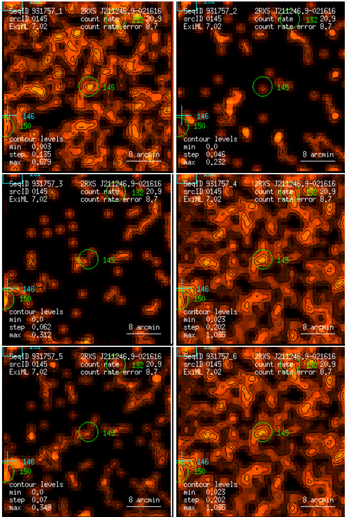
Figure 145: RASS 931757: detection 0145: band rate images, Gaussian filter: (1) PSPC channels 11 – 41, (2) 52 – 90, (3) 91 – 201, (4) 11 – 235, (5) 52 – 201, (6) 11 – 201. Broad band rates in counts/ks. Band rate contour levels in counts/ks/arcmin 2 .
