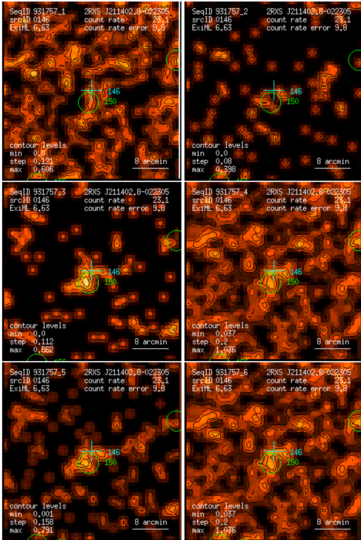
Figure 146: RASS 931757: detection 0146: band rate images, Gaussian filter: (1) PSPC channels 11 – 41, (2) 52 – 90, (3) 91 – 201, (4) 11 – 235, (5) 52 – 201, (6) 11 – 201. Broad band rates in counts/ks. Band rate contour levels in counts/ks/arcmin 2 .
