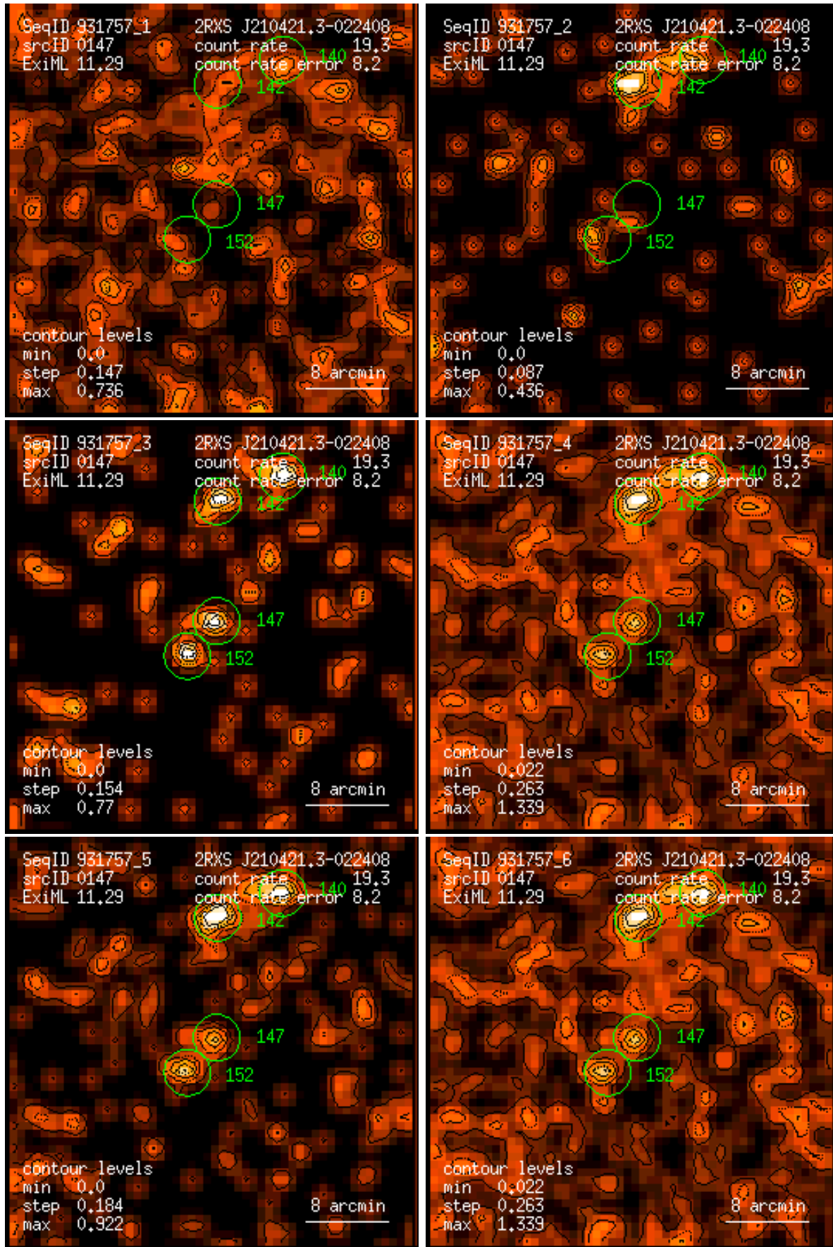
Figure 147: RASS 931757: detection 0147: band rate images, Gaussian filter: (1) PSPC channels 11 – 41, (2) 52 – 90, (3) 91 – 201, (4) 11 – 235, (5) 52 – 201, (6) 11 – 201. Broad band rates in counts/ks. Band rate contour levels in counts/ks/arcmin 2 .
