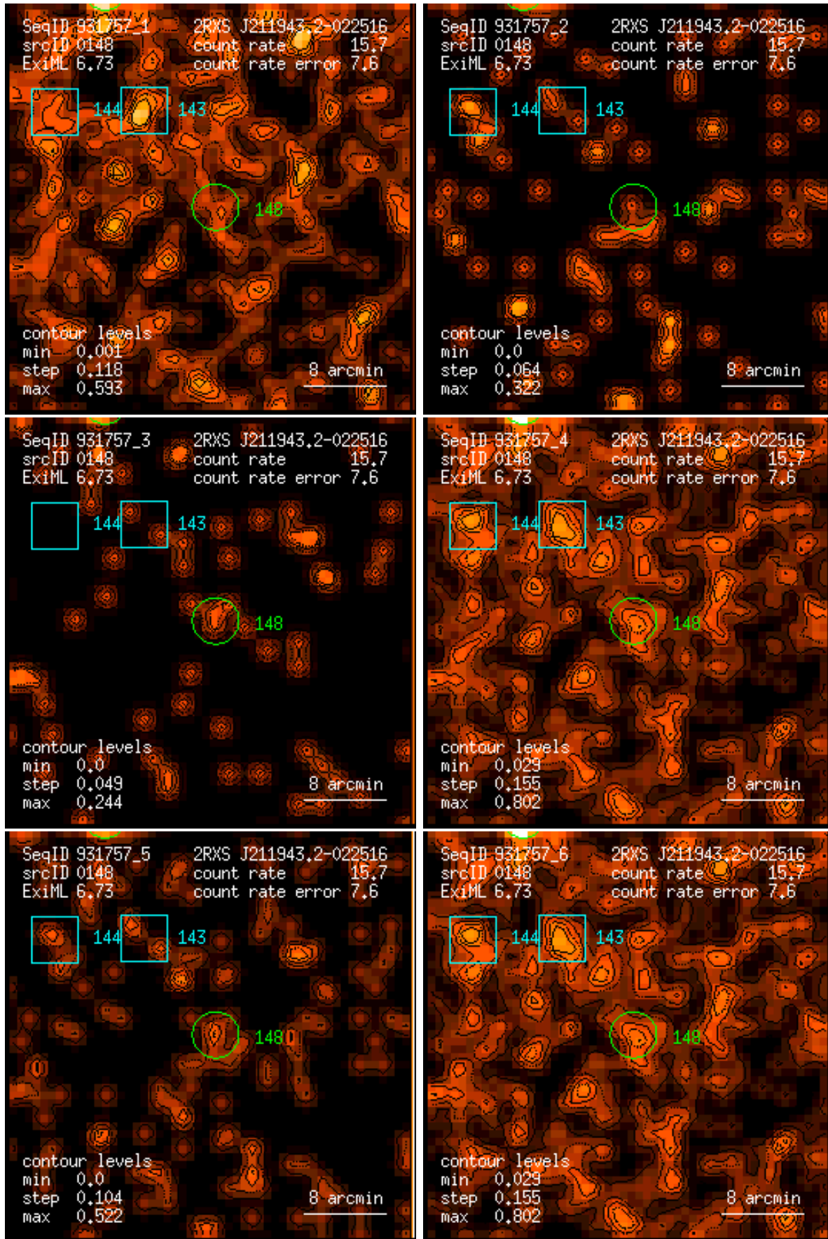
Figure 148: RASS 931757: detection 0148: band rate images, Gaussian filter: (1) PSPC channels 11 – 41, (2) 52 – 90, (3) 91 – 201, (4) 11 – 235, (5) 52 – 201, (6) 11 – 201. Broad band rates in counts/ks. Band rate contour levels in counts/ks/arcmin 2 .
