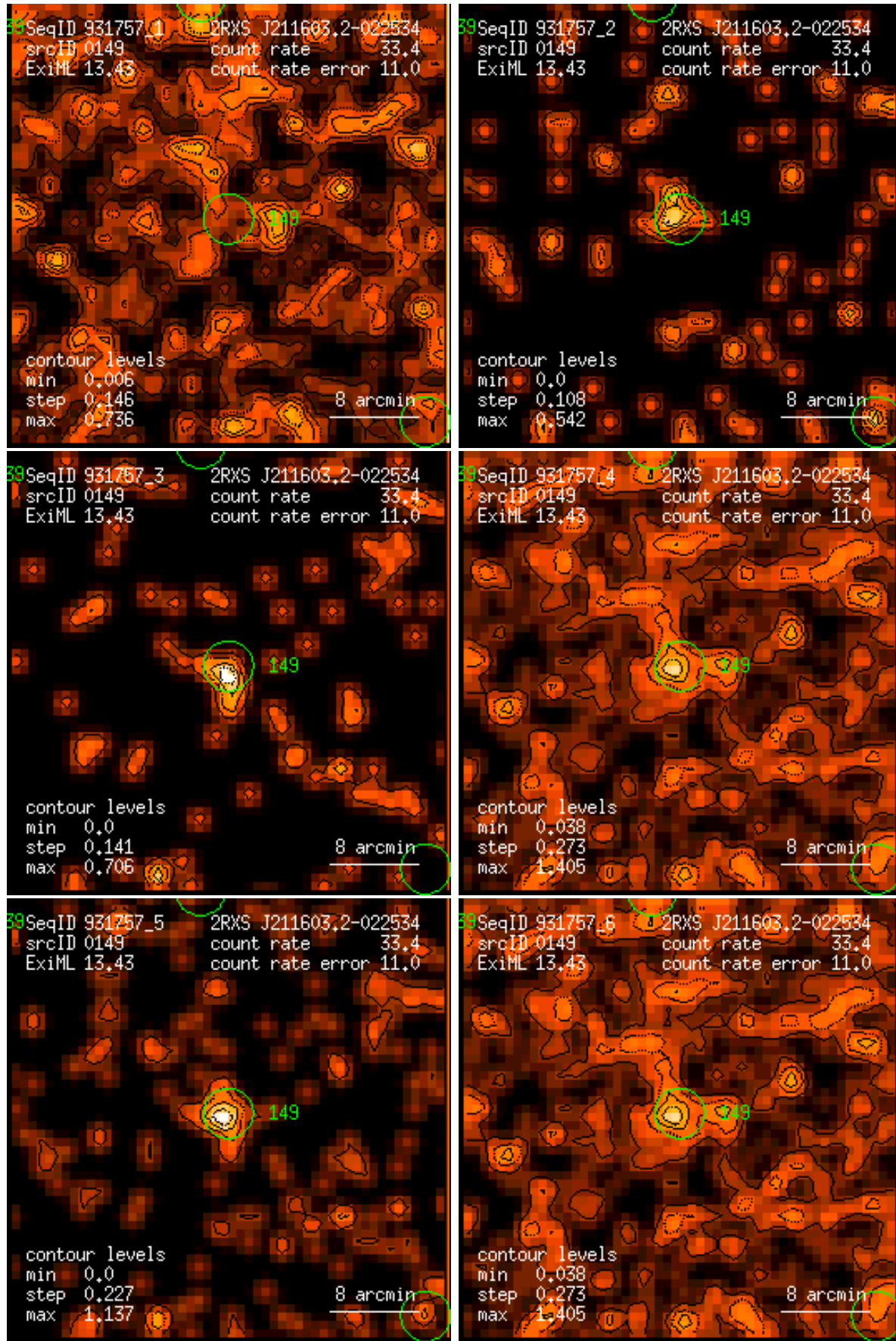
Figure 149: RASS 931757: detection 0149: band rate images, Gaussian filter: (1) PSPC channels 11 – 41, (2) 52 – 90, (3) 91 – 201, (4) 11 – 235, (5) 52 – 201, (6) 11 – 201. Broad band rates in counts/ks. Band rate contour levels in counts/ks/arcmin 2 .
