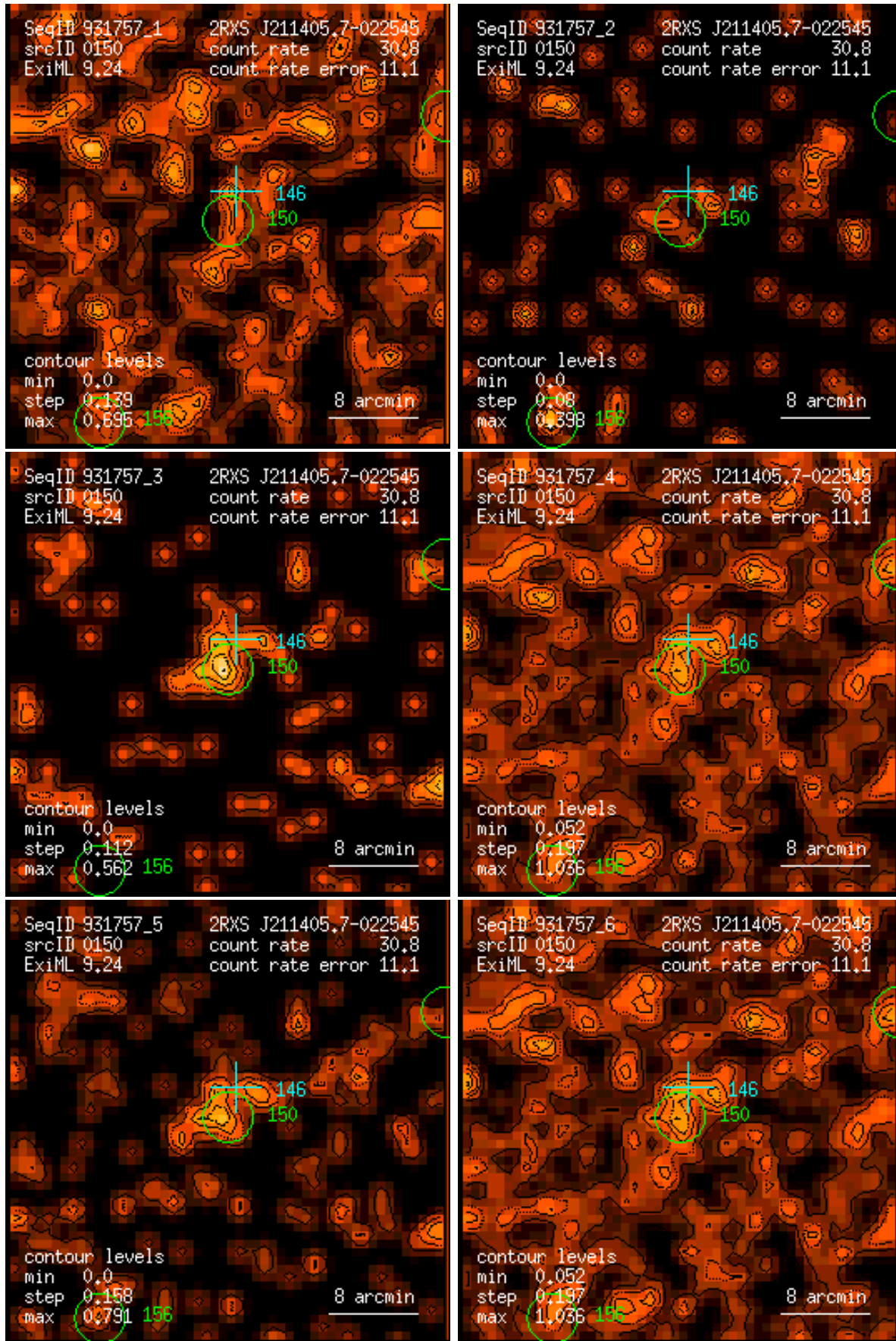
Figure 150: RASS 931757: detection 0150: band rate images, Gaussian filter: (1) PSPC channels 11 – 41, (2) 52 – 90, (3) 91 – 201, (4) 11 – 235, (5) 52 – 201, (6) 11 – 201. Broad band rates in counts/ks. Band rate contour levels in counts/ks/arcmin 2 .
