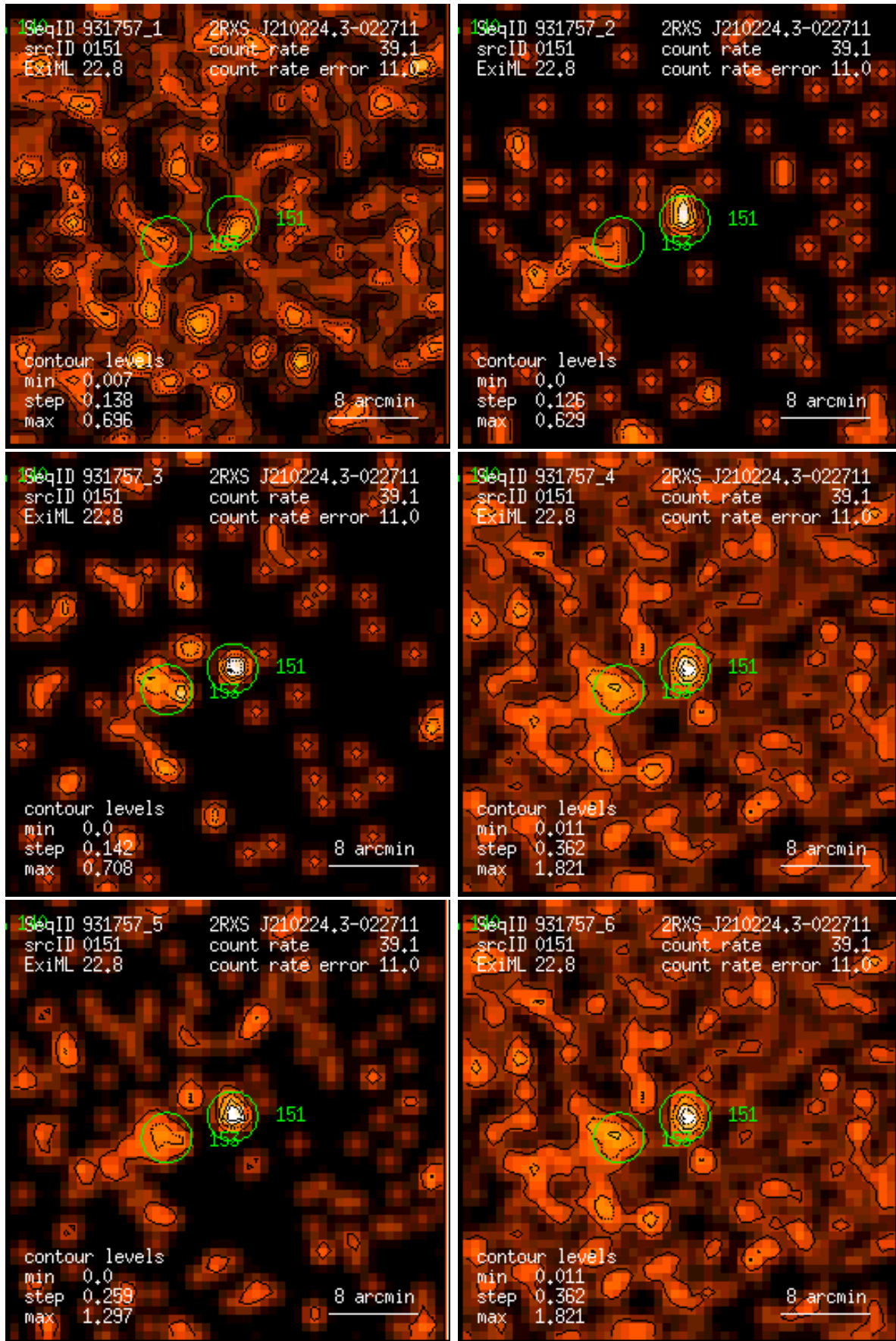
Figure 151: RASS 931757: detection 0151: band rate images, Gaussian filter: (1) PSPC channels 11 – 41, (2) 52 – 90, (3) 91 – 201, (4) 11 – 235, (5) 52 – 201, (6) 11 – 201. Broad band rates in counts/ks. Band rate contour levels in counts/ks/arcmin 2 .
