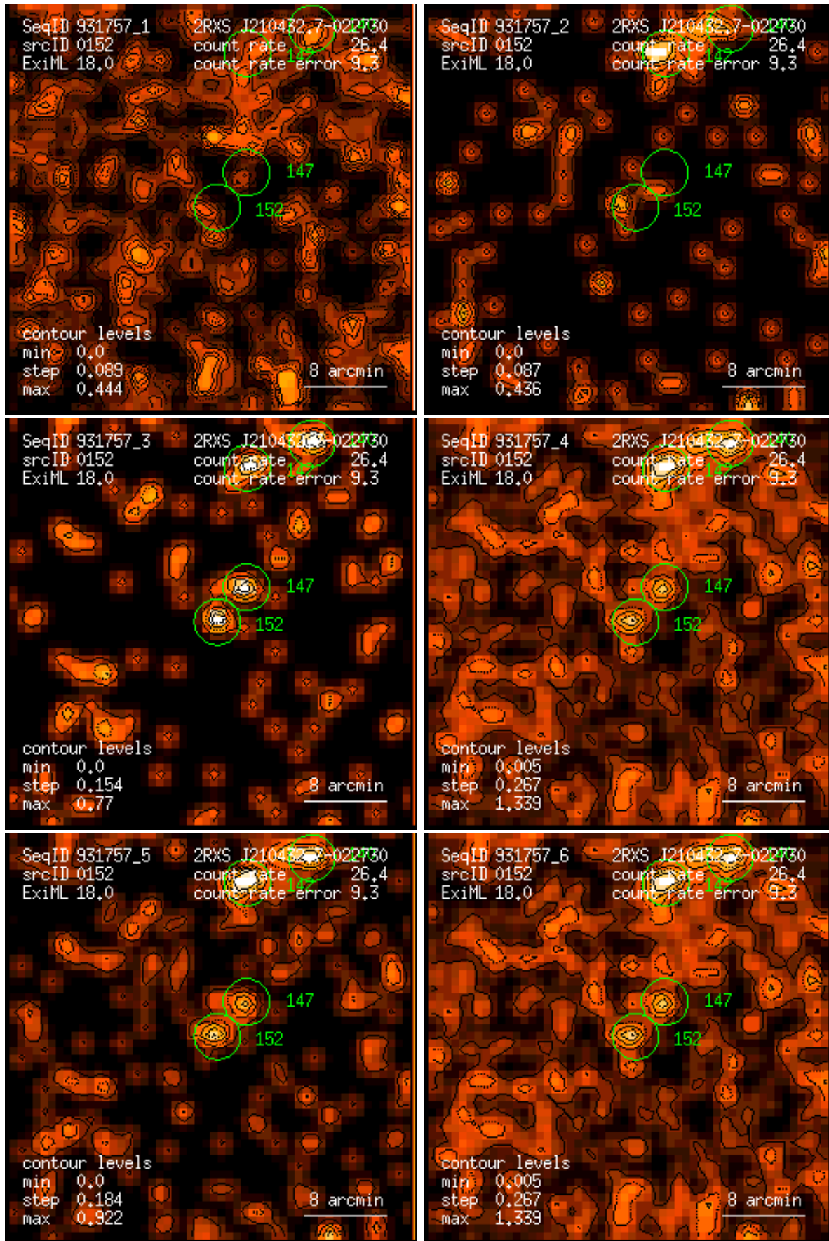
Figure 152: RASS 931757: detection 0152: band rate images, Gaussian filter: (1) PSPC channels 11 – 41, (2) 52 – 90, (3) 91 – 201, (4) 11 – 235, (5) 52 – 201, (6) 11 – 201. Broad band rates in counts/ks. Band rate contour levels in counts/ks/arcmin 2 .
