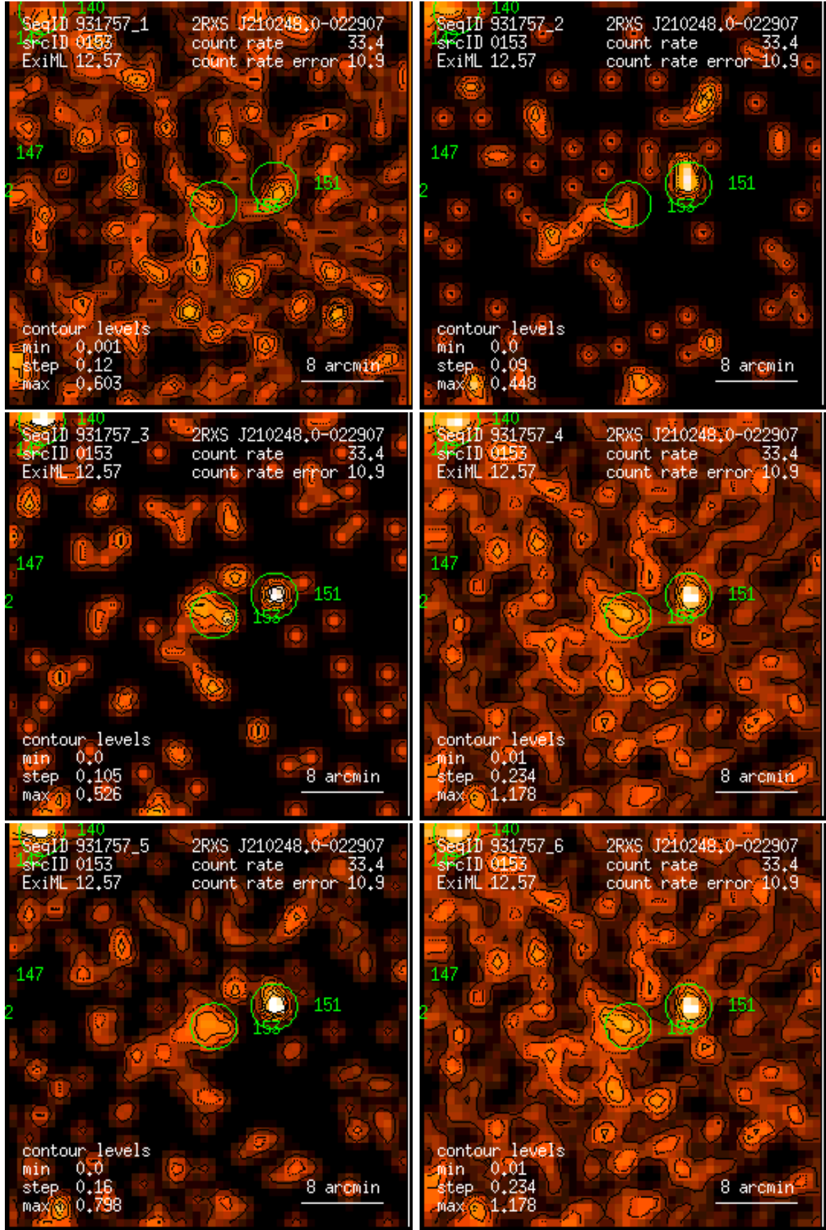
Figure 153: RASS 931757: detection 0153: band rate images, Gaussian filter: (1) PSPC channels 11 – 41, (2) 52 – 90, (3) 91 – 201, (4) 11 – 235, (5) 52 – 201, (6) 11 – 201. Broad band rates in counts/ks. Band rate contour levels in counts/ks/arcmin 2 .
