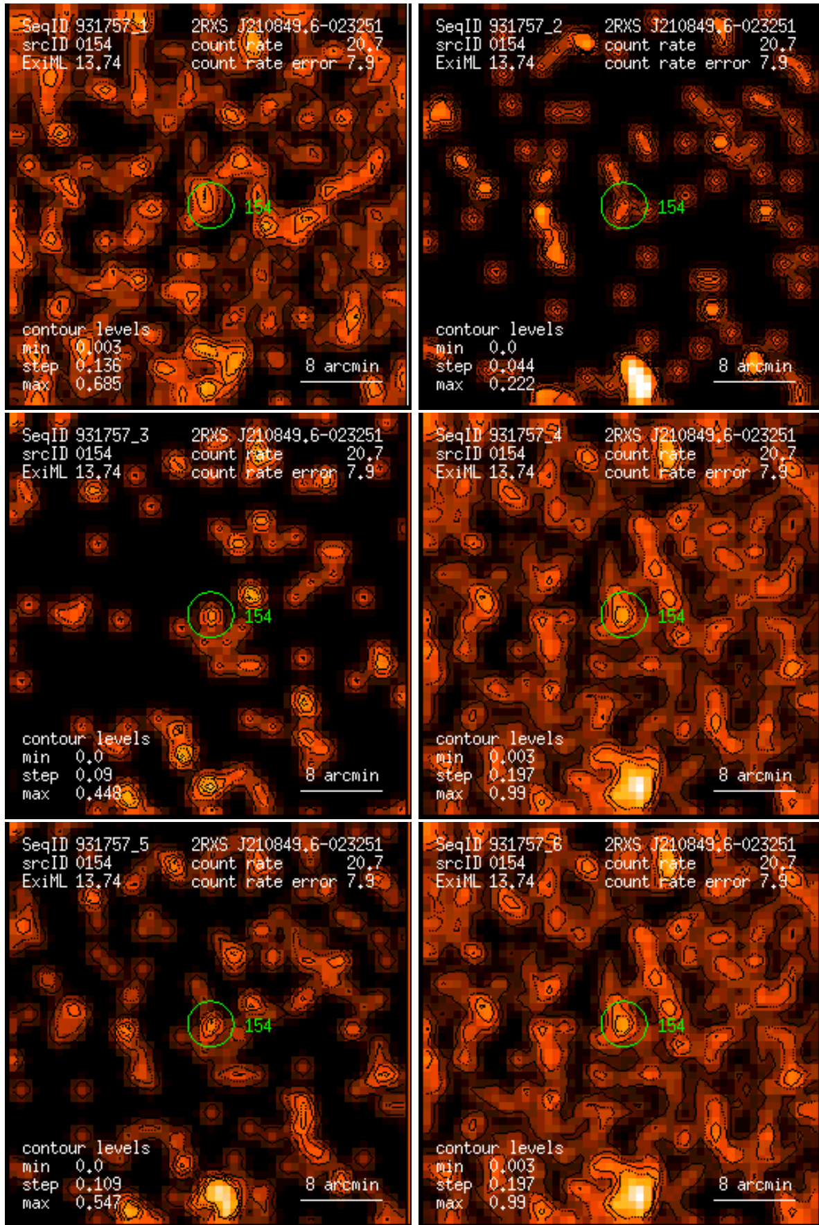
Figure 154: RASS 931757: detection 0154: band rate images, Gaussian filter: (1) PSPC channels 11 – 41, (2) 52 – 90, (3) 91 – 201, (4) 11 – 235, (5) 52 – 201, (6) 11 – 201. Broad band rates in counts/ks. Band rate contour levels in counts/ks/arcmin 2 .
