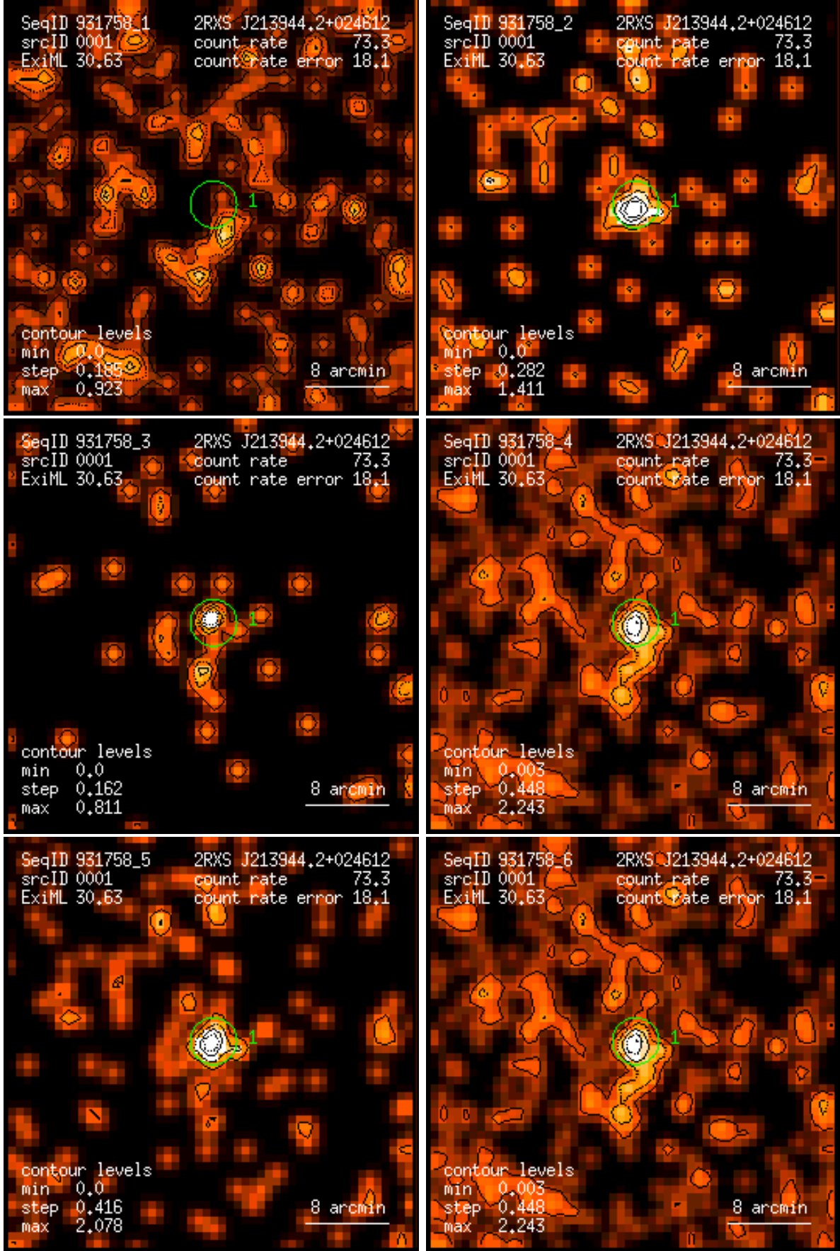
Figure 1: RASS 931758: detection 0001: band rate images, Gaussian filter: (1) PSPC channels 11 – 41, (2) 52 – 90, (3) 91 – 201, (4) 11 – 235, (5) 52 – 201, (6) 11 – 201. Broad band rates in counts/ks. Band rate contour levels in counts/ks/arcmin 2 .
