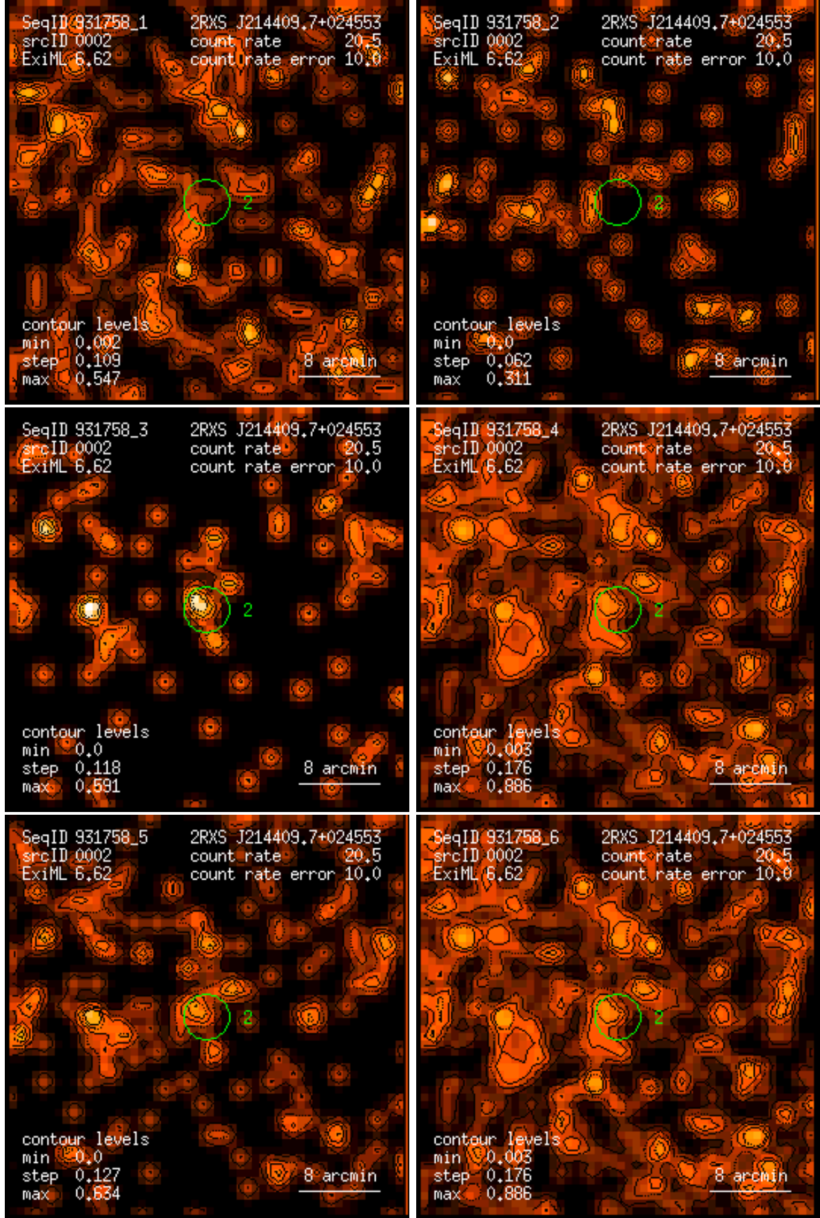
Figure 2: RASS 931758: detection 0002: band rate images, Gaussian filter: (1) PSPC channels 11 – 41, (2) 52 – 90, (3) 91 – 201, (4) 11 – 235, (5) 52 – 201, (6) 11 – 201. Broad band rates in counts/ks. Band rate contour levels in counts/ks/arcmin 2 .
