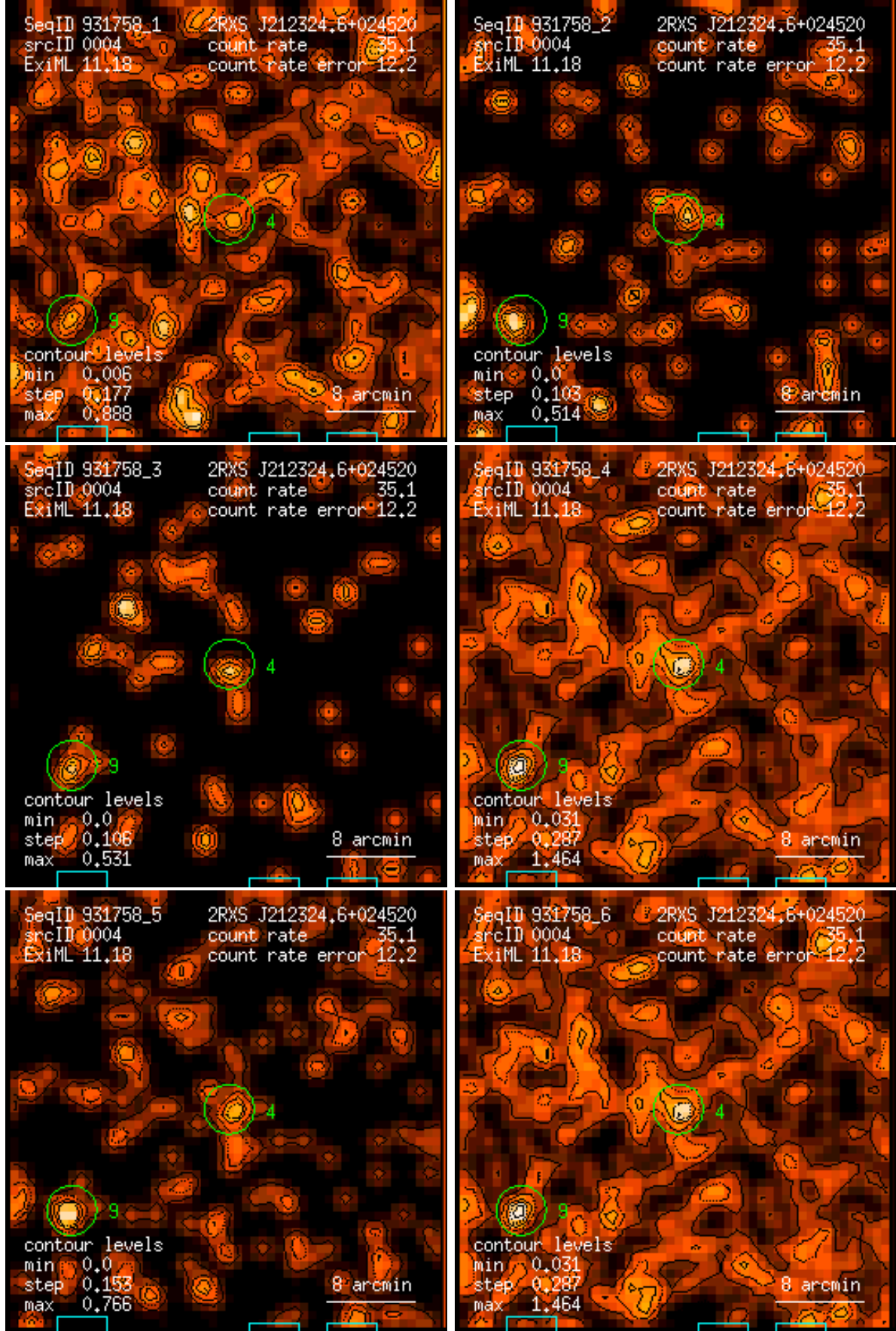
Figure 4: RASS 931758: detection 0004: band rate images, Gaussian filter: (1) PSPC channels 11 – 41, (2) 52 – 90, (3) 91 – 201, (4) 11 – 235, (5) 52 – 201, (6) 11 – 201. Broad band rates in counts/ks. Band rate contour levels in counts/ks/arcmin 2 .
