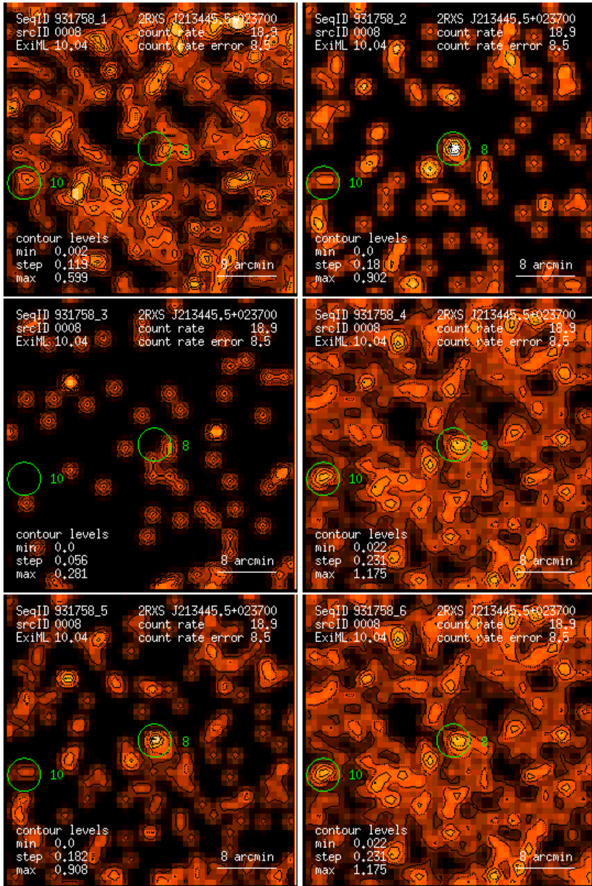
Figure 8: RASS 931758: detection 0008: band rate images, Gaussian filter: (1) PSPC channels 11 – 41, (2) 52 – 90, (3) 91 – 201, (4) 11 – 235, (5) 52 – 201, (6) 11 – 201. Broad band rates in counts/ks. Band rate contour levels in counts/ks/arcmin 2 .
