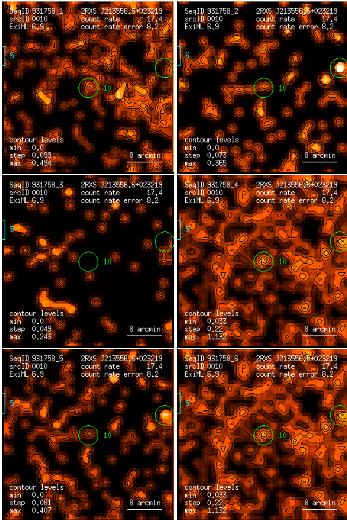
Figure 10: RASS 931758: detection 0010: band rate images, Gaussian filter: (1) PSPC channels 11 – 41, (2) 52 – 90, (3) 91 – 201, (4) 11 – 235, (5) 52 – 201, (6) 11 – 201. Broad band rates in counts/ks. Band rate contour levels in counts/ks/arcmin 2 .
