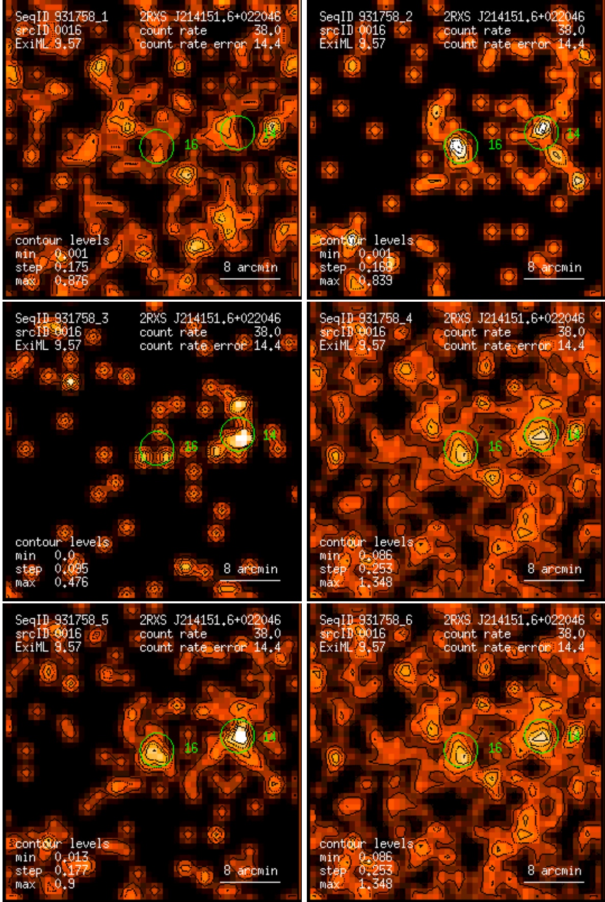
Figure 16: RASS 931758: detection 0016: band rate images, Gaussian filter: (1) PSPC channels 11 – 41, (2) 52 – 90, (3) 91 – 201, (4) 11 – 235, (5) 52 – 201, (6) 11 – 201. Broad band rates in counts/ks. Band rate contour levels in counts/ks/arcmin 2 .
