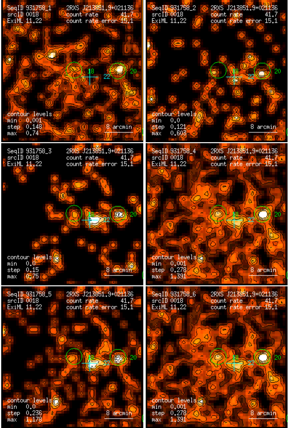
Figure 18: RASS 931758: detection 0018: band rate images, Gaussian filter: (1) PSPC channels 11 – 41, (2) 52 – 90, (3) 91 – 201, (4) 11 – 235, (5) 52 – 201, (6) 11 – 201. Broad band rates in counts/ks. Band rate contour levels in counts/ks/arcmin 2 .
