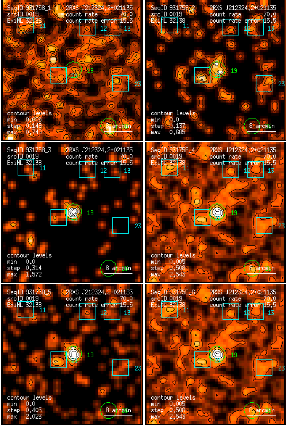
Figure 19: RASS 931758: detection 0019: band rate images, Gaussian filter: (1) PSPC channels 11 – 41, (2) 52 – 90, (3) 91 – 201, (4) 11 – 235, (5) 52 – 201, (6) 11 – 201. Broad band rates in counts/ks. Band rate contour levels in counts/ks/arcmin 2 .
