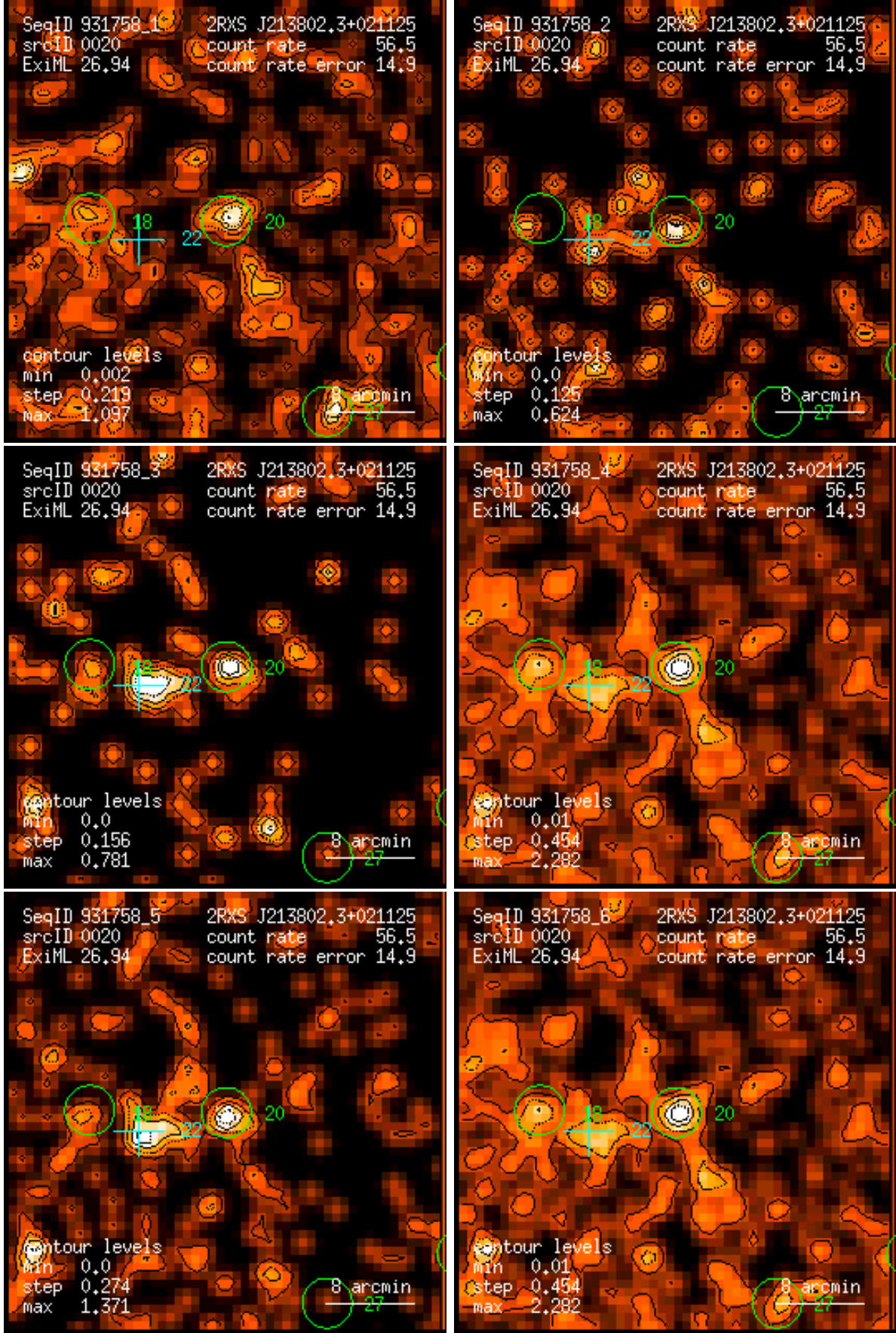
Figure 20: RASS 931758: detection 0020: band rate images, Gaussian filter: (1) PSPC channels 11 – 41, (2) 52 – 90, (3) 91 – 201, (4) 11 – 235, (5) 52 – 201, (6) 11 – 201. Broad band rates in counts/ks. Band rate contour levels in counts/ks/arcmin 2 .
