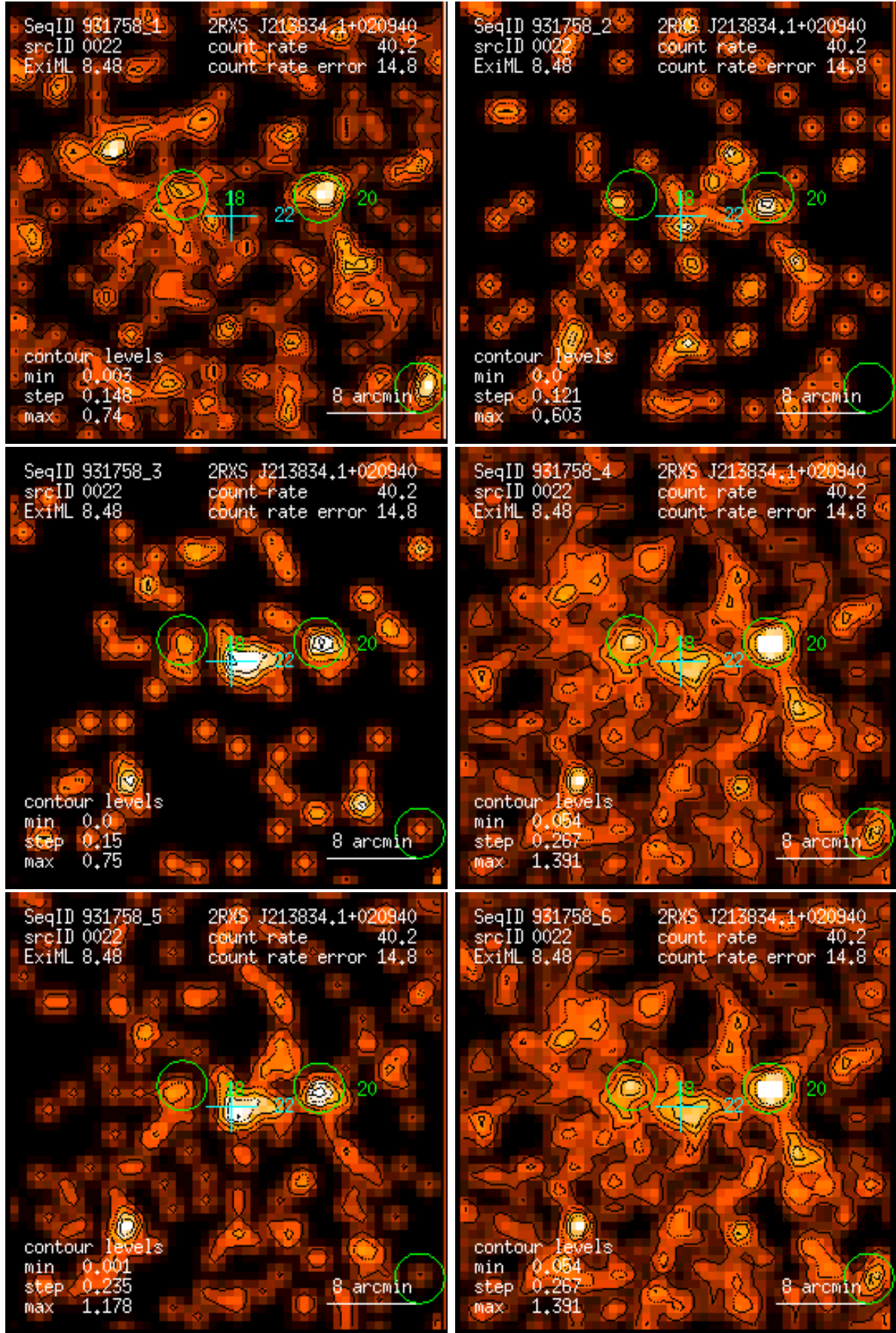
Figure 22: RASS 931758: detection 0022: band rate images, Gaussian filter: (1) PSPC channels 11 – 41, (2) 52 – 90, (3) 91 – 201, (4) 11 – 235, (5) 52 – 201, (6) 11 – 201. Broad band rates in counts/ks. Band rate contour levels in counts/ks/arcmin 2 .
