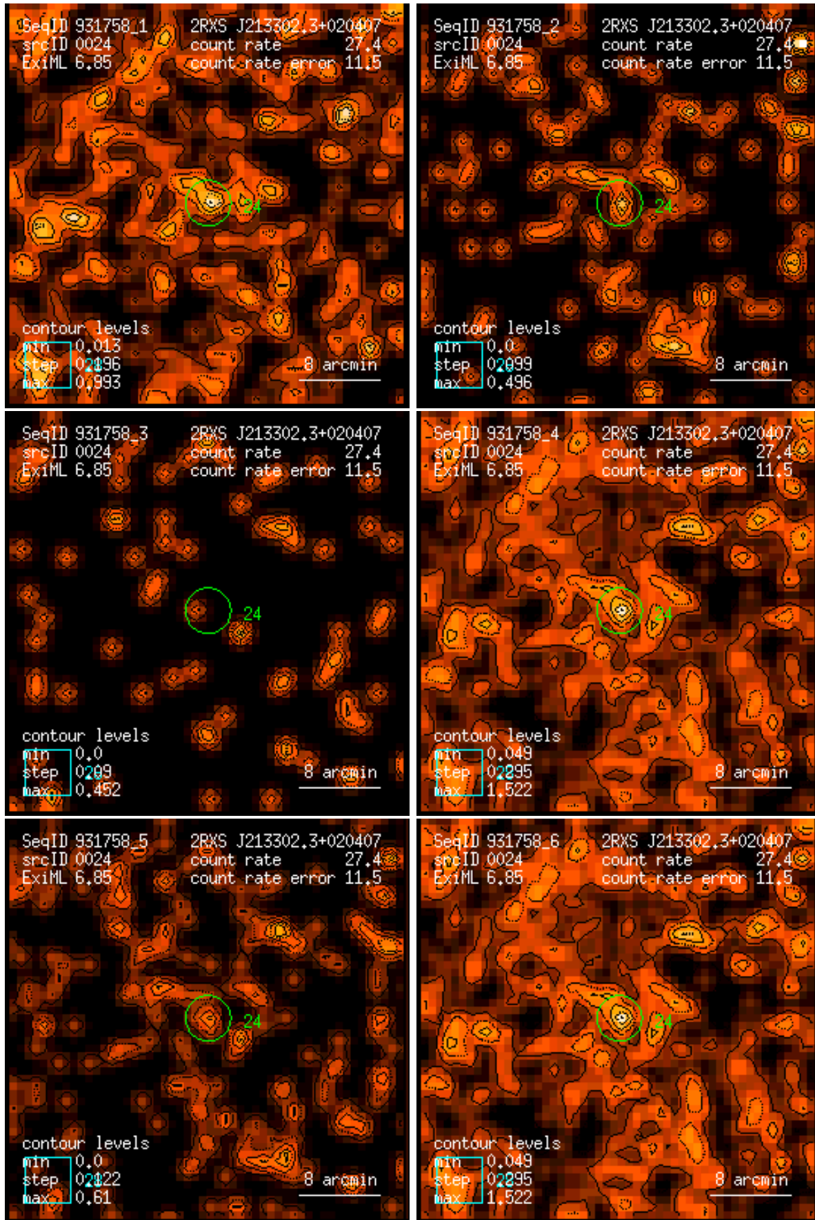
Figure 24: RASS 931758: detection 0024: band rate images, Gaussian filter: (1) PSPC channels 11 – 41, (2) 52 – 90, (3) 91 – 201, (4) 11 – 235, (5) 52 – 201, (6) 11 – 201. Broad band rates in counts/ks. Band rate contour levels in counts/ks/arcmin 2 .
