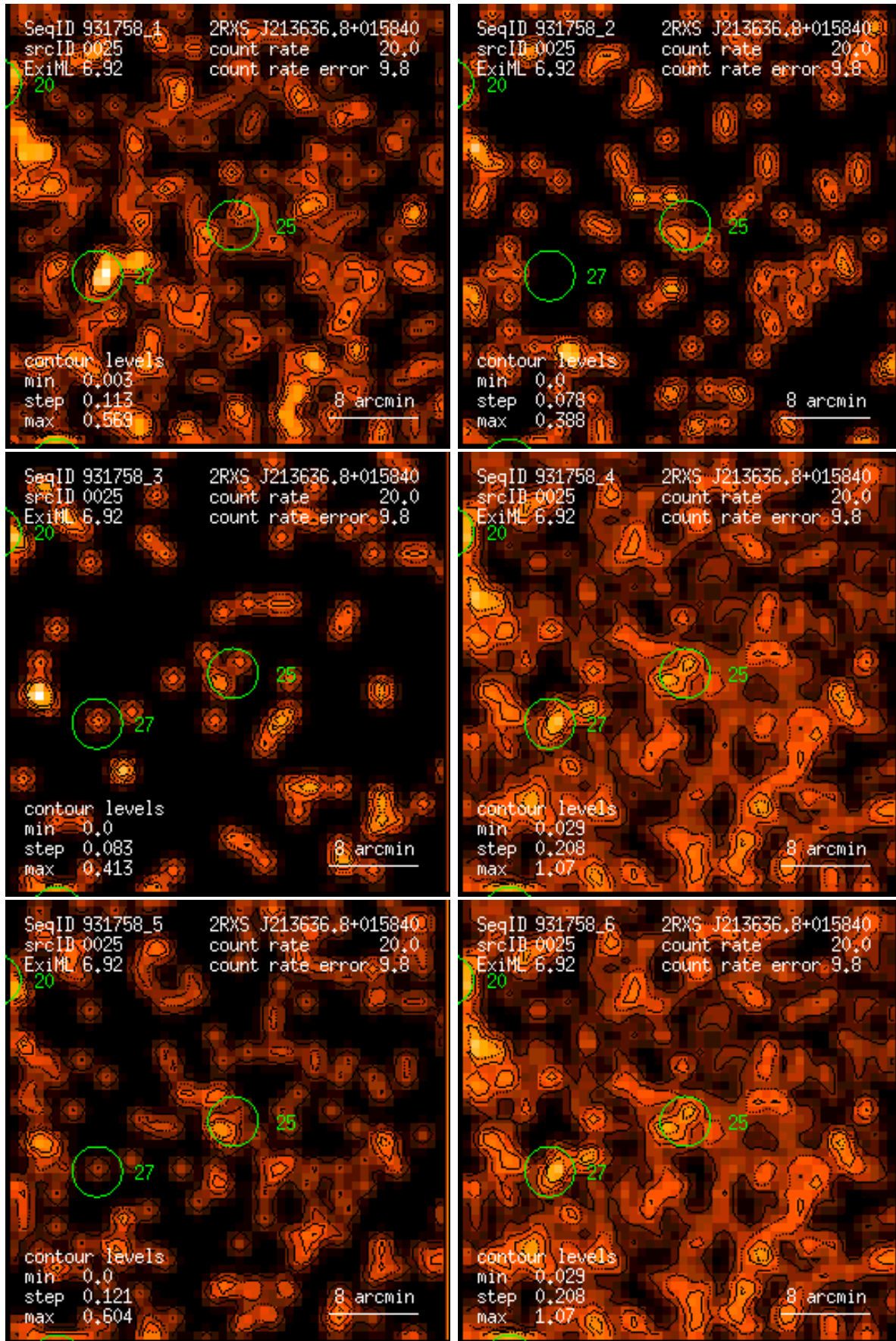
Figure 25: RASS 931758: detection 0025: band rate images, Gaussian filter: (1) PSPC channels 11 – 41, (2) 52 – 90, (3) 91 – 201, (4) 11 – 235, (5) 52 – 201, (6) 11 – 201. Broad band rates in counts/ks. Band rate contour levels in counts/ks/arcmin 2 .
