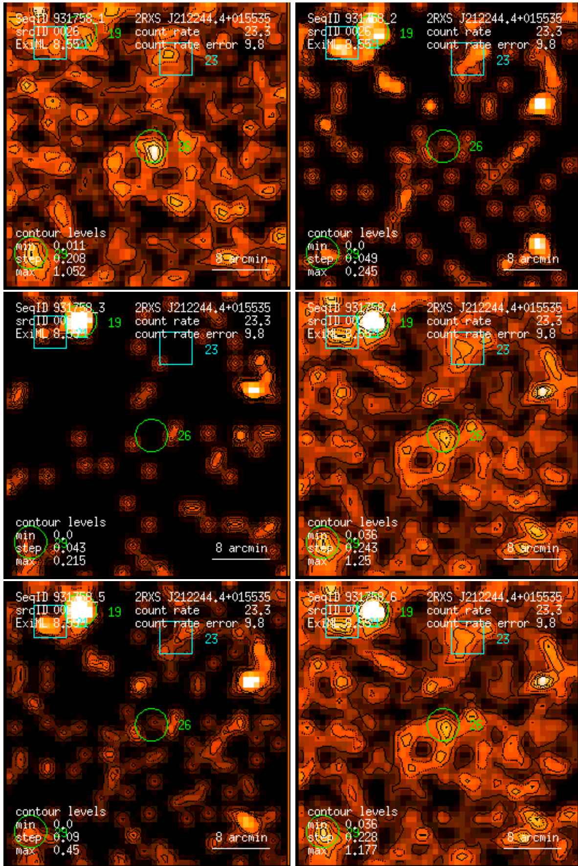
Figure 26: RASS 931758: detection 0026: band rate images, Gaussian filter: (1) PSPC channels 11 – 41, (2) 52 – 90, (3) 91 – 201, (4) 11 – 235, (5) 52 – 201, (6) 11 – 201. Broad band rates in counts/ks. Band rate contour levels in counts/ks/arcmin 2 .
