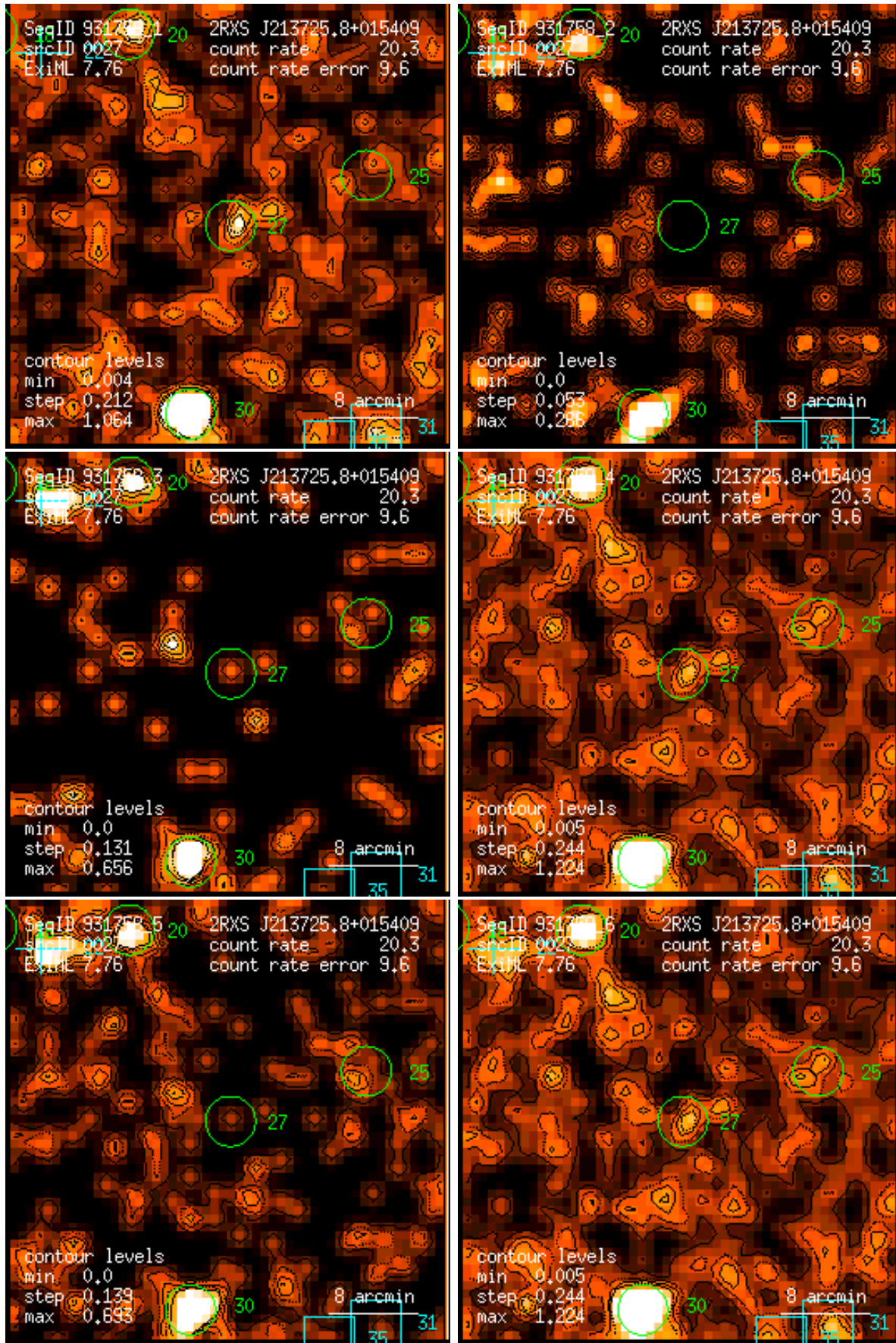
Figure 27: RASS 931758: detection 0027: band rate images, Gaussian filter: (1) PSPC channels 11 – 41, (2) 52 – 90, (3) 91 – 201, (4) 11 – 235, (5) 52 – 201, (6) 11 – 201. Broad band rates in counts/ks. Band rate contour levels in counts/ks/arcmin 2 .
