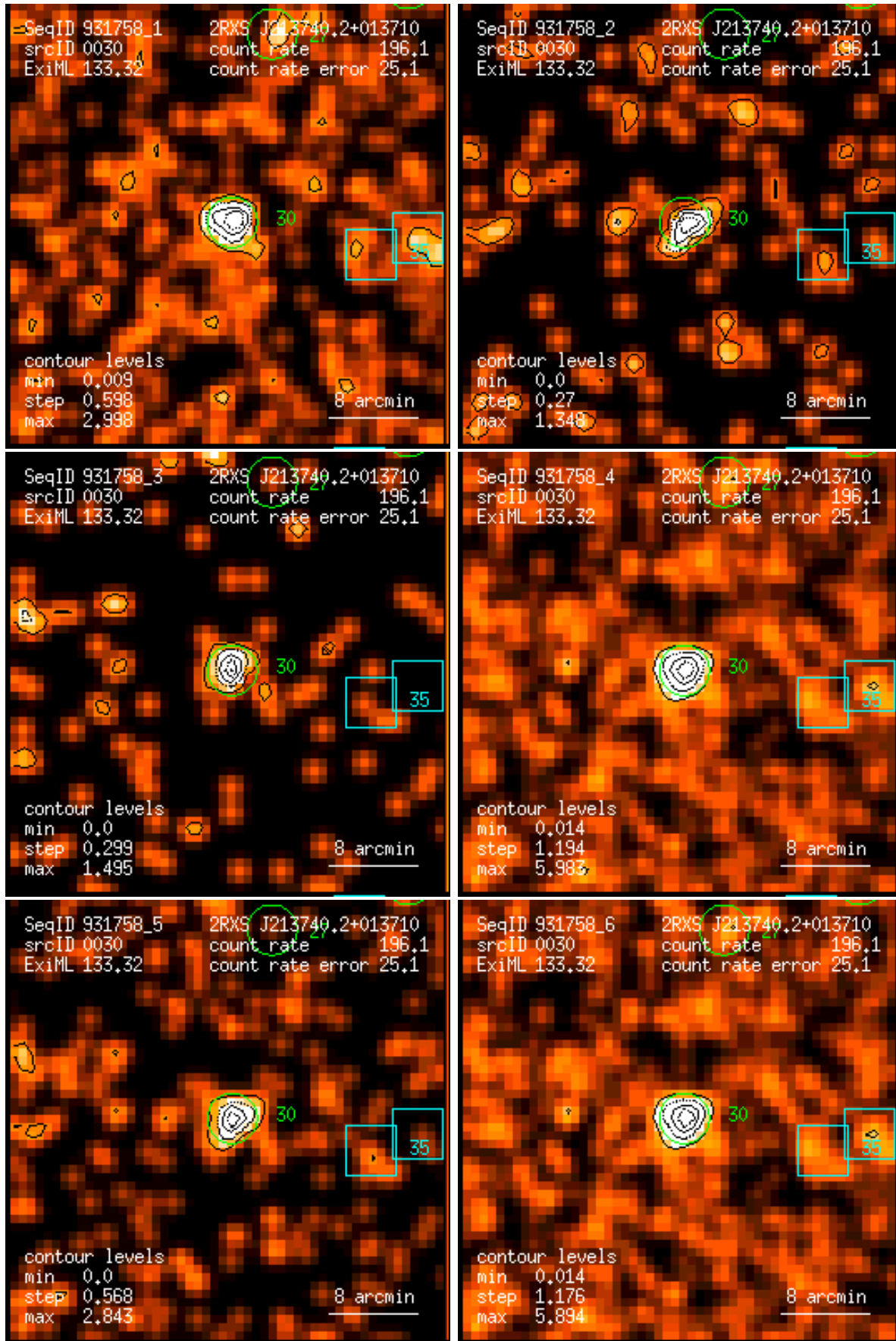
Figure 30: RASS 931758: detection 0030: band rate images, Gaussian filter: (1) PSPC channels 11 – 41, (2) 52 – 90, (3) 91 – 201, (4) 11 – 235, (5) 52 – 201, (6) 11 – 201. Broad band rates in counts/ks. Band rate contour levels in counts/ks/arcmin 2 .
