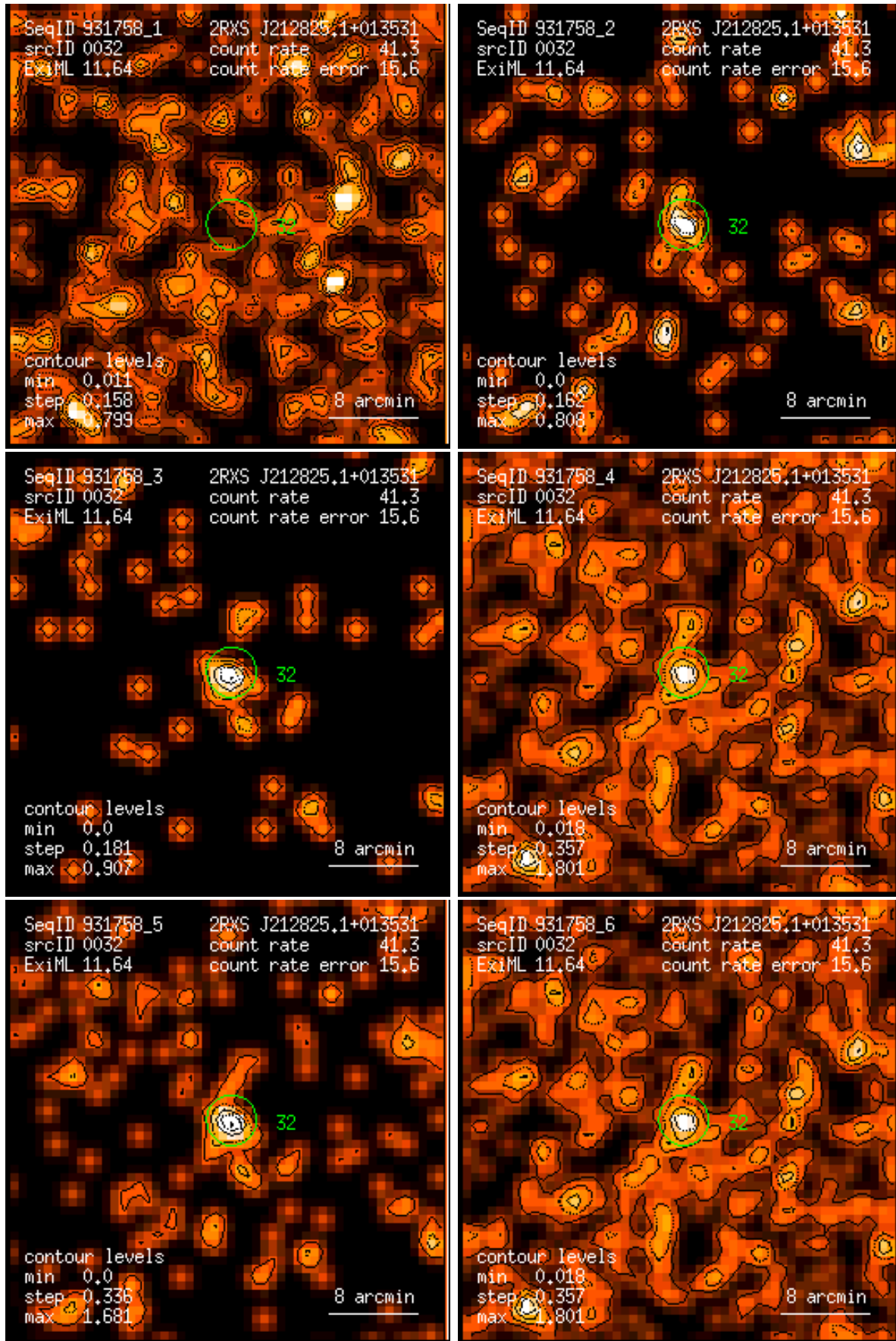
Figure 32: RASS 931758: detection 0032: band rate images, Gaussian filter: (1) PSPC channels 11 – 41, (2) 52 – 90, (3) 91 – 201, (4) 11 – 235, (5) 52 – 201, (6) 11 – 201. Broad band rates in counts/ks. Band rate contour levels in counts/ks/arcmin 2 .
