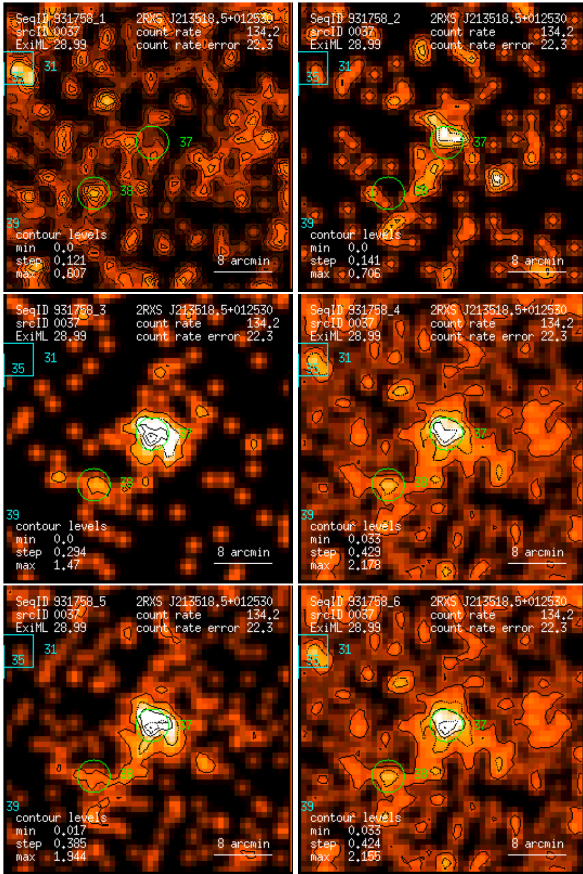
Figure 37: RASS 931758: detection 0037: band rate images, Gaussian filter: (1) PSPC channels 11 – 41, (2) 52 – 90, (3) 91 – 201, (4) 11 – 235, (5) 52 – 201, (6) 11 – 201. Broad band rates in counts/ks. Band rate contour levels in counts/ks/arcmin 2 .
