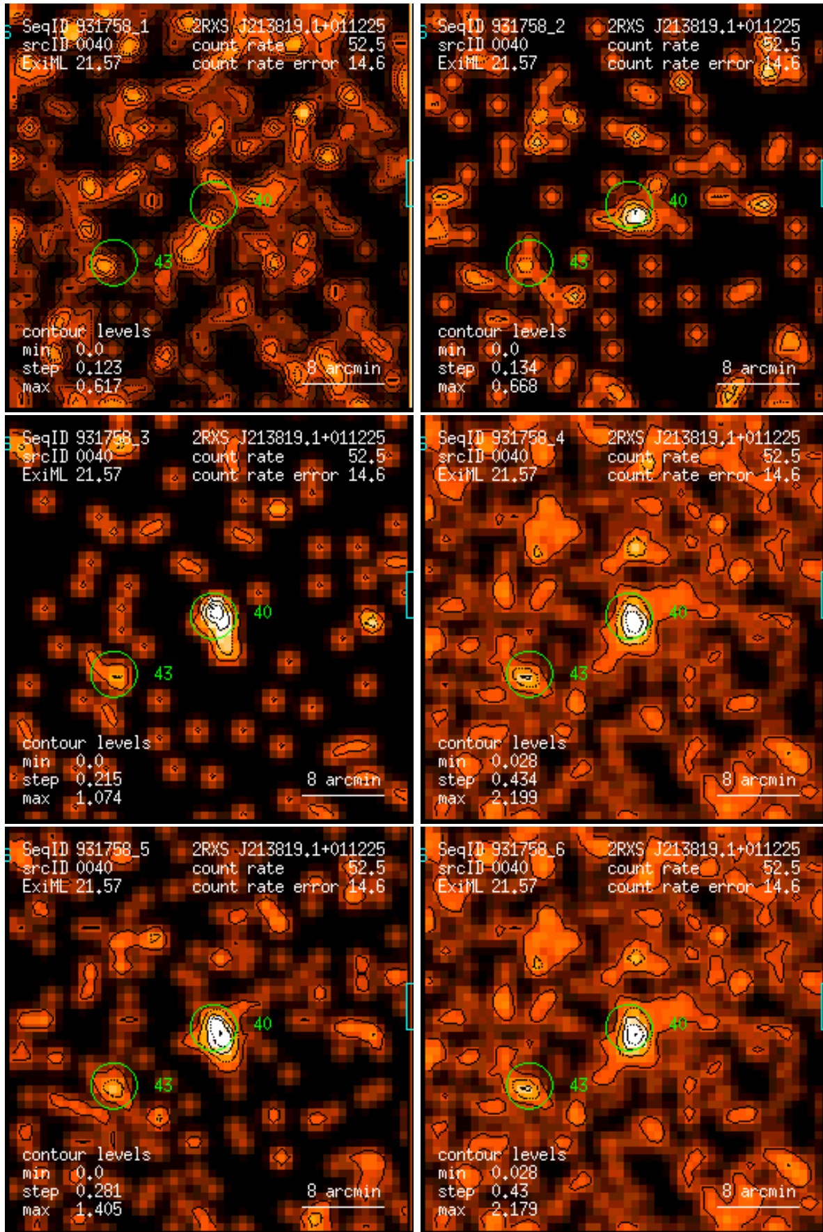
Figure 40: RASS 931758: detection 0040: band rate images, Gaussian filter: (1) PSPC channels 11 – 41, (2) 52 – 90, (3) 91 – 201, (4) 11 – 235, (5) 52 – 201, (6) 11 – 201. Broad band rates in counts/ks. Band rate contour levels in counts/ks/arcmin 2 .
