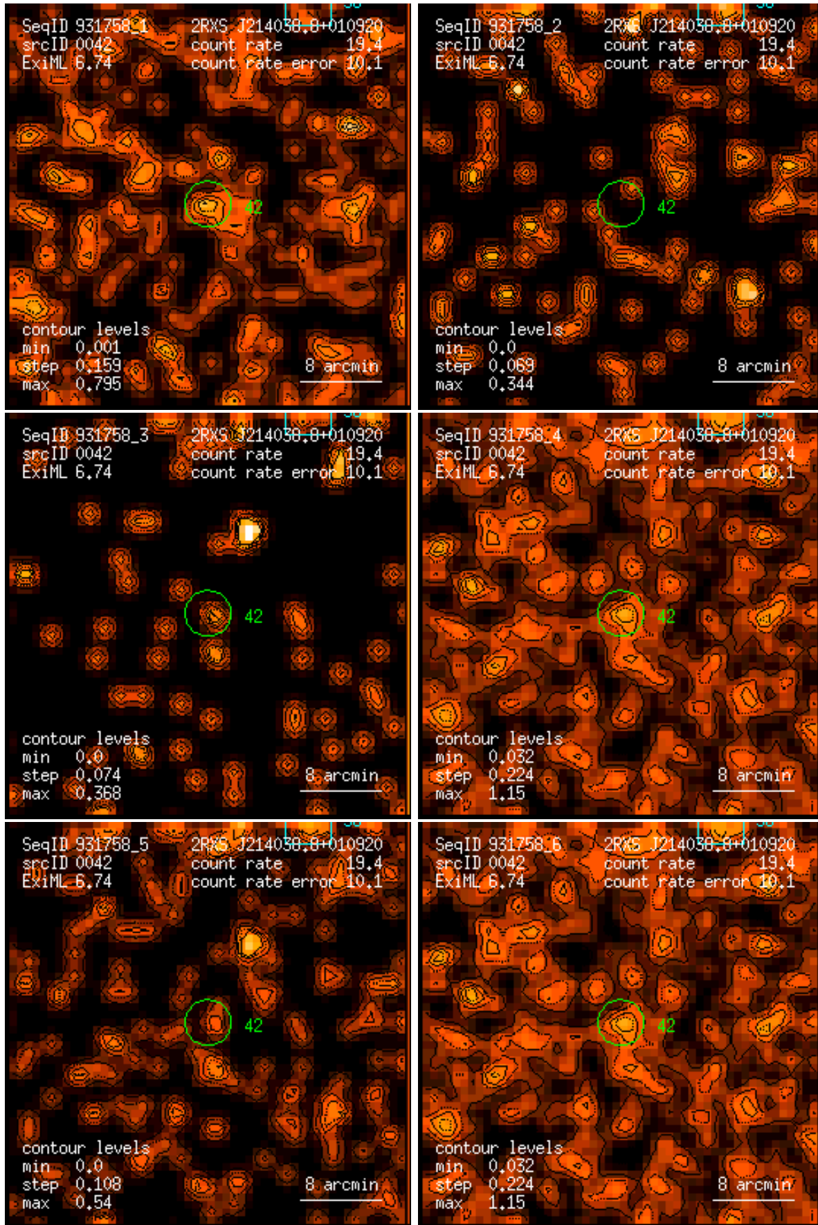
Figure 42: RASS 931758: detection 0042: band rate images, Gaussian filter: (1) PSPC channels 11 – 41, (2) 52 – 90, (3) 91 – 201, (4) 11 – 235, (5) 52 – 201, (6) 11 – 201. Broad band rates in counts/ks. Band rate contour levels in counts/ks/arcmin 2 .
