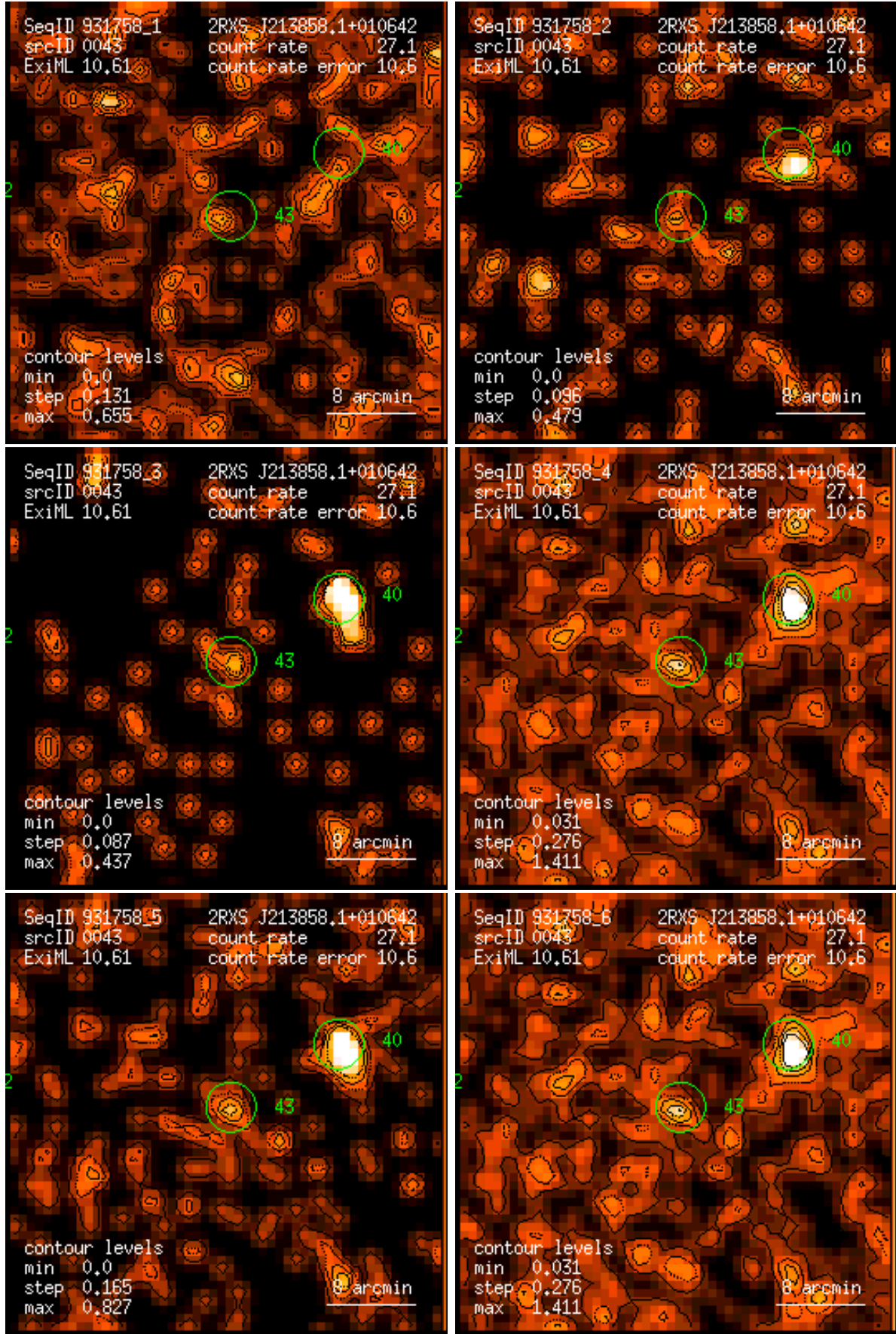
Figure 43: RASS 931758: detection 0043: band rate images, Gaussian filter: (1) PSPC channels 11 – 41, (2) 52 – 90, (3) 91 – 201, (4) 11 – 235, (5) 52 – 201, (6) 11 – 201. Broad band rates in counts/ks. Band rate contour levels in counts/ks/arcmin 2 .
