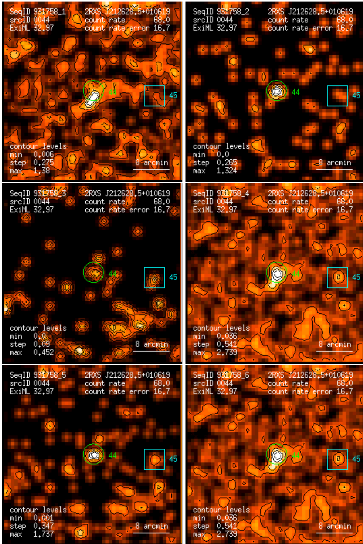
Figure 44: RASS 931758: detection 0044: band rate images, Gaussian filter: (1) PSPC channels 11 – 41, (2) 52 – 90, (3) 91 – 201, (4) 11 – 235, (5) 52 – 201, (6) 11 – 201. Broad band rates in counts/ks. Band rate contour levels in counts/ks/arcmin 2 .
