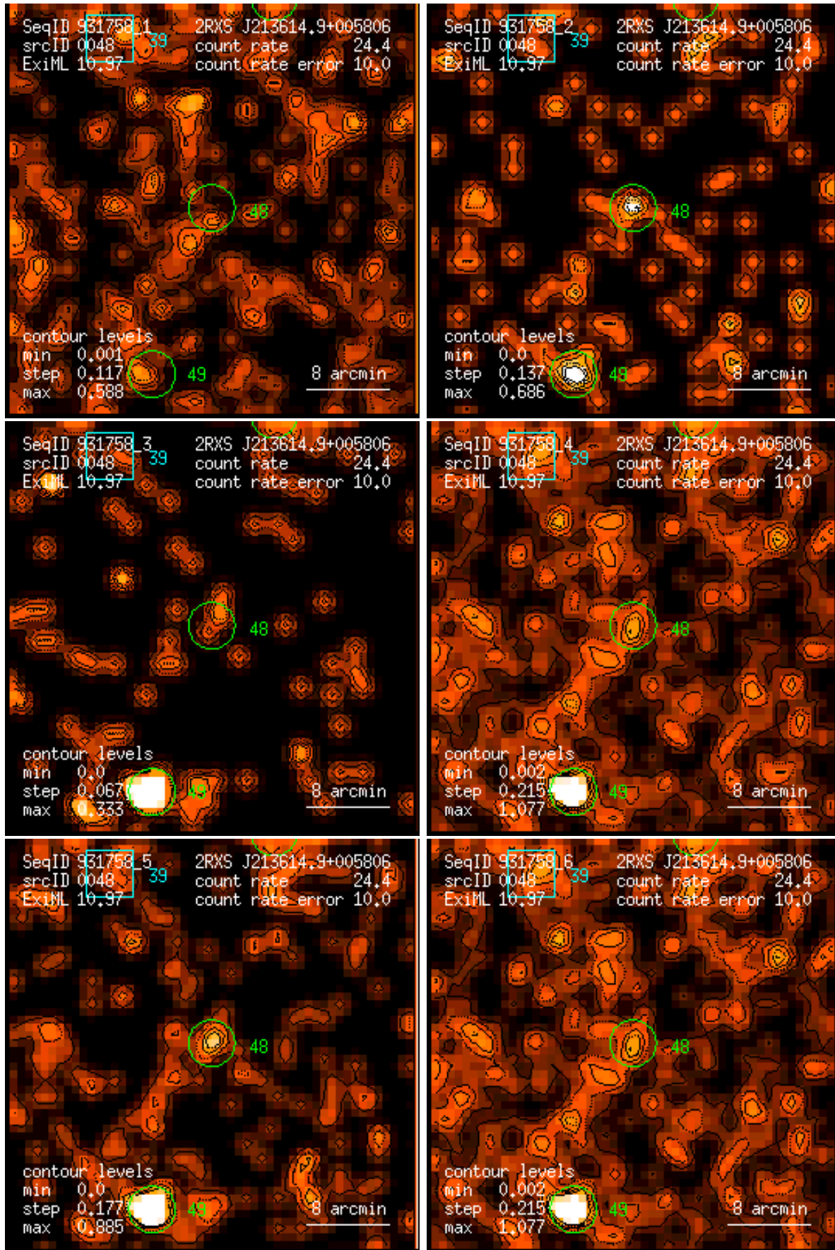
Figure 48: RASS 931758: detection 0048: band rate images, Gaussian filter: (1) PSPC channels 11 – 41, (2) 52 – 90, (3) 91 – 201, (4) 11 – 235, (5) 52 – 201, (6) 11 – 201. Broad band rates in counts/ks. Band rate contour levels in counts/ks/arcmin 2 .
