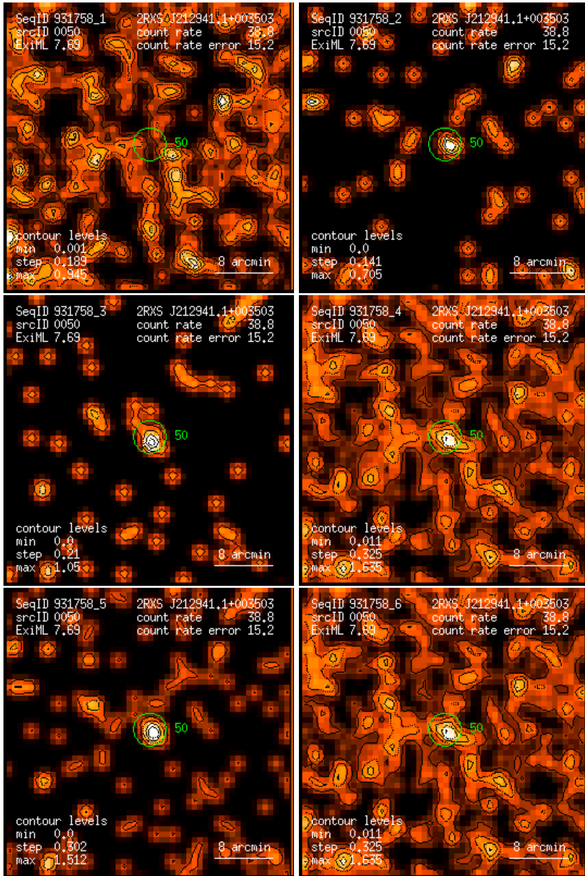
Figure 50: RASS 931758: detection 0050: band rate images, Gaussian filter: (1) PSPC channels 11 – 41, (2) 52 – 90, (3) 91 – 201, (4) 11 – 235, (5) 52 – 201, (6) 11 – 201. Broad band rates in counts/ks. Band rate contour levels in counts/ks/arcmin 2 .
