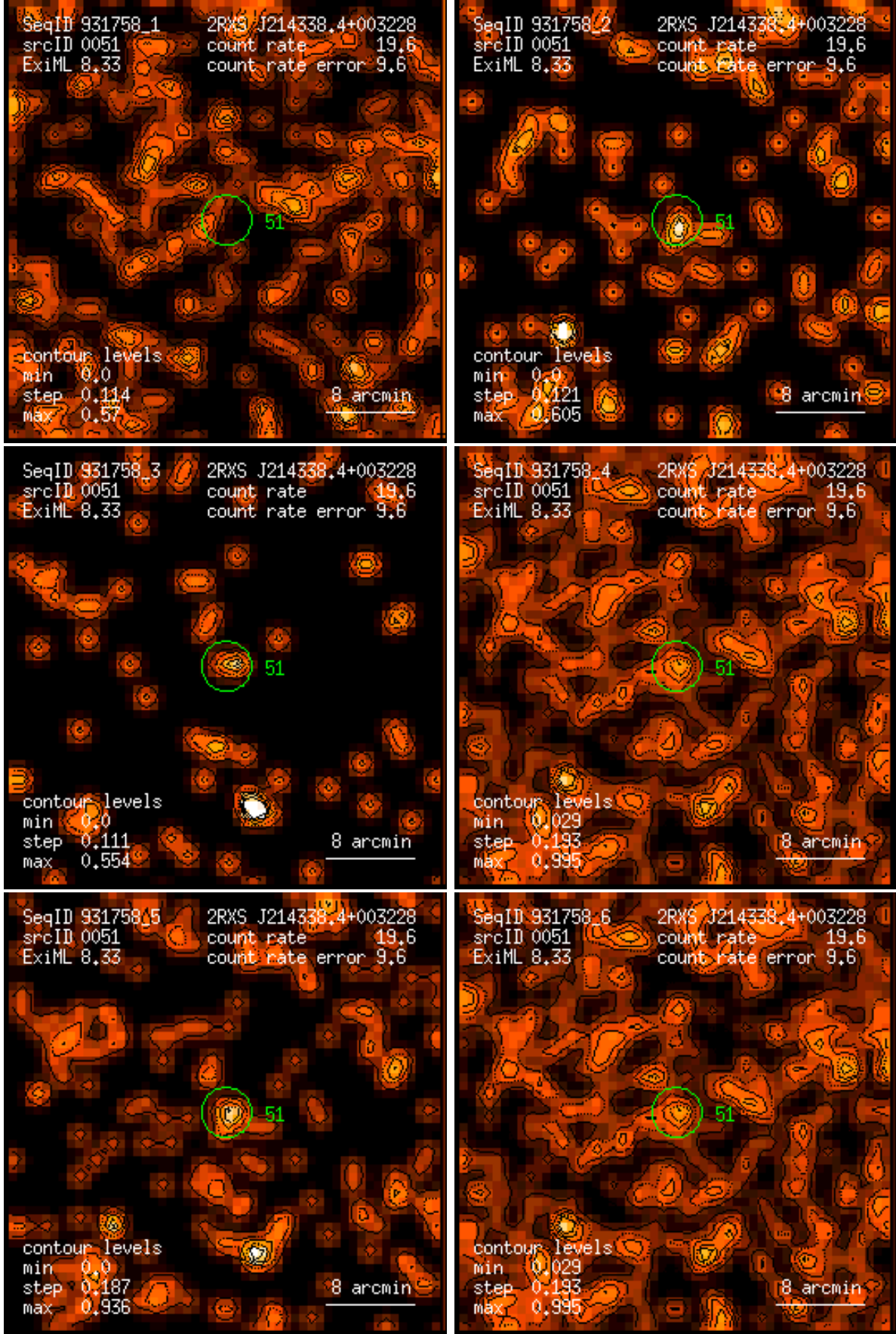
Figure 51: RASS 931758: detection 0051: band rate images, Gaussian filter: (1) PSPC channels 11 – 41, (2) 52 – 90, (3) 91 – 201, (4) 11 – 235, (5) 52 – 201, (6) 11 – 201. Broad band rates in counts/ks. Band rate contour levels in counts/ks/arcmin 2 .
