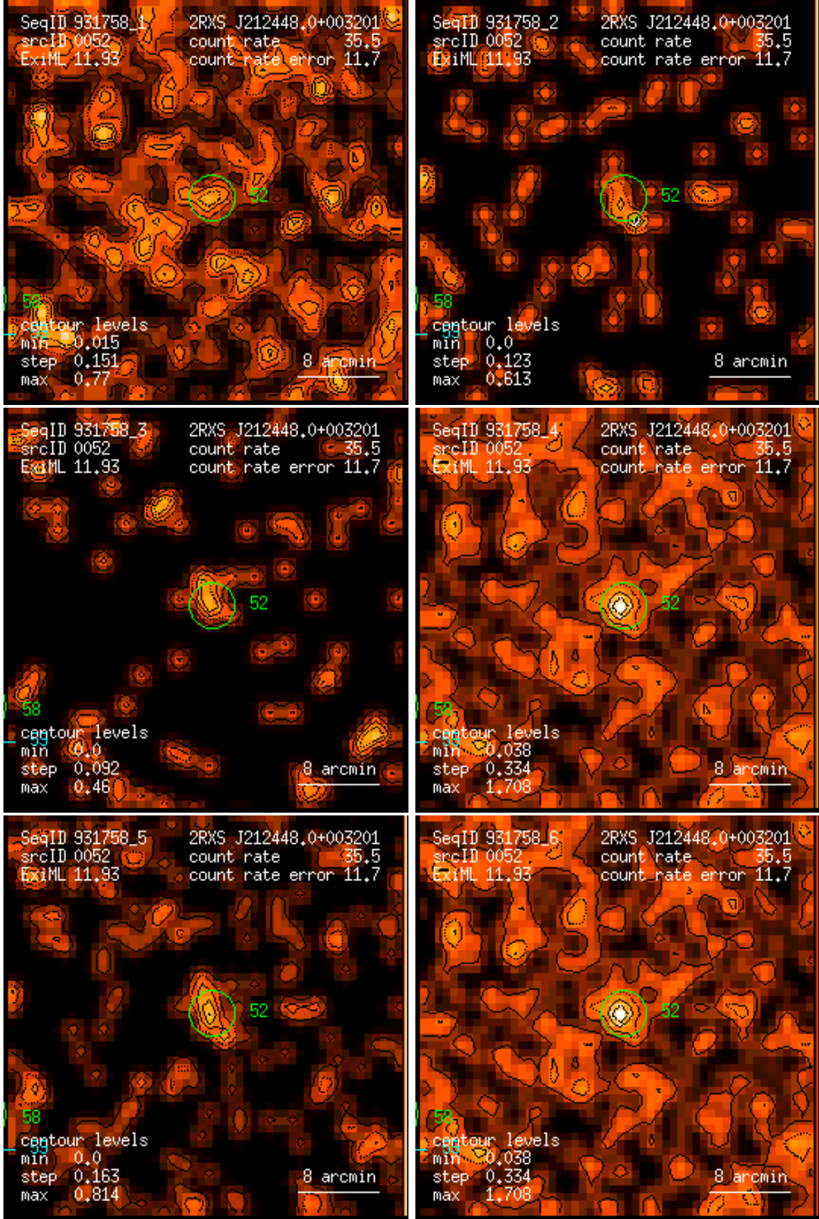
Figure 52: RASS 931758: detection 0052: band rate images, Gaussian filter: (1) PSPC channels 11 – 41, (2) 52 – 90, (3) 91 – 201, (4) 11 – 235, (5) 52 – 201, (6) 11 – 201. Broad band rates in counts/ks. Band rate contour levels in counts/ks/arcmin 2 .
