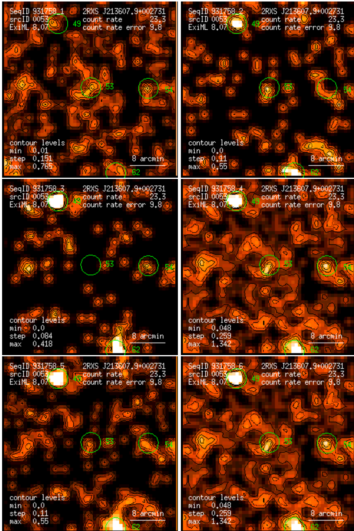
Figure 53: RASS 931758: detection 0053: band rate images, Gaussian filter: (1) PSPC channels 11 – 41, (2) 52 – 90, (3) 91 – 201, (4) 11 – 235, (5) 52 – 201, (6) 11 – 201. Broad band rates in counts/ks. Band rate contour levels in counts/ks/arcmin 2 .
