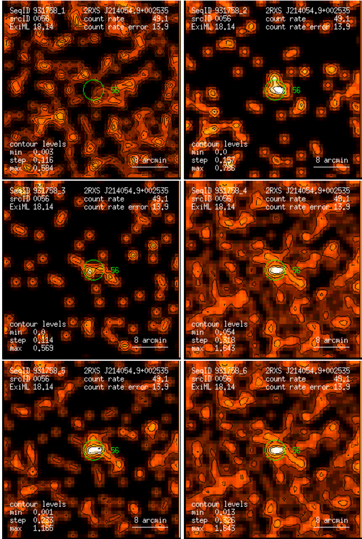
Figure 56: RASS 931758: detection 0056: band rate images, Gaussian filter: (1) PSPC channels 11 – 41, (2) 52 – 90, (3) 91 – 201, (4) 11 – 235, (5) 52 – 201, (6) 11 – 201. Broad band rates in counts/ks. Band rate contour levels in counts/ks/arcmin 2 .
