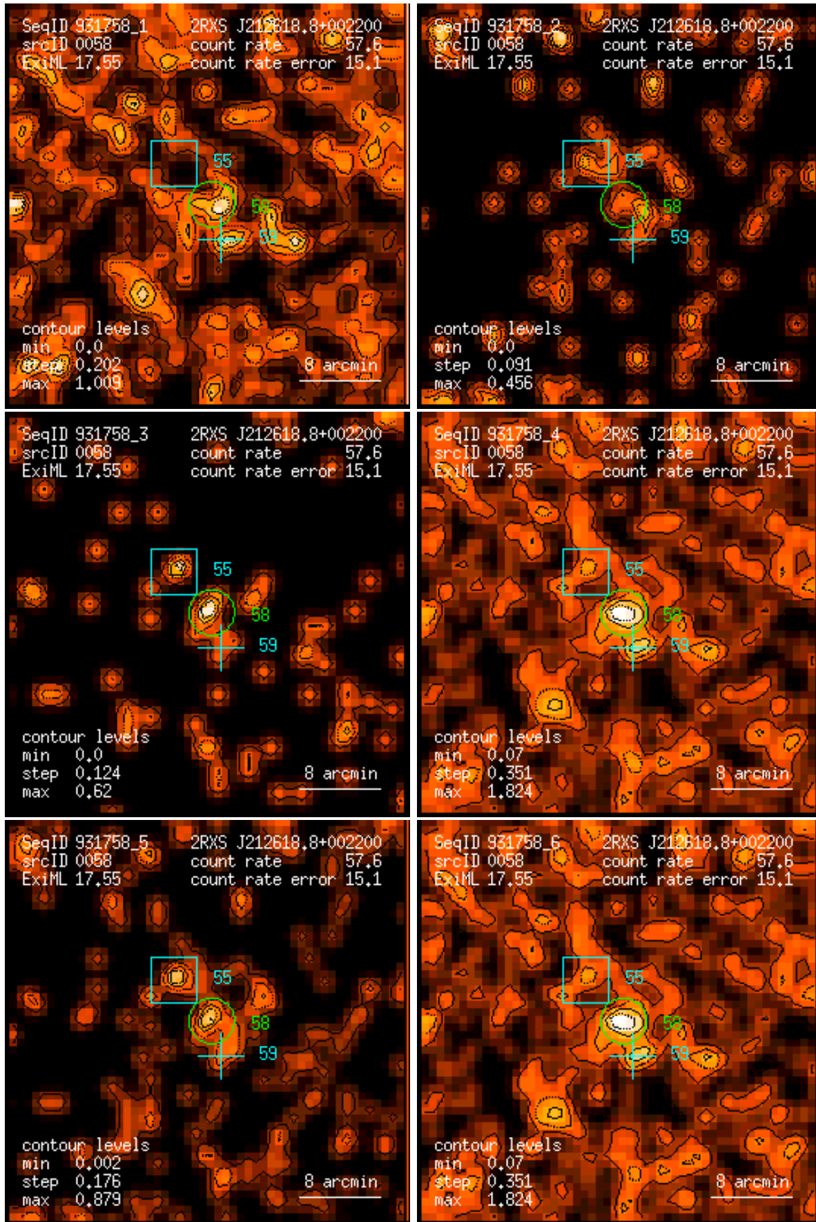
Figure 58: RASS 931758: detection 0058: band rate images, Gaussian filter: (1) PSPC channels 11 – 41, (2) 52 – 90, (3) 91 – 201, (4) 11 – 235, (5) 52 – 201, (6) 11 – 201. Broad band rates in counts/ks. Band rate contour levels in counts/ks/arcmin 2 .
